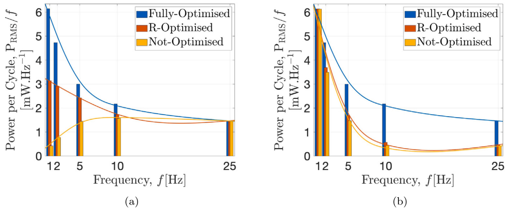
Fig. 12. Comparison between non-optimised, R-optimised, and fully-optimised sliding-mode triboelectric harvesters considering the optimal parameters from the (a) 50 mm at 25 Hz and (b) 50 mm at 1 Hz configurations.
