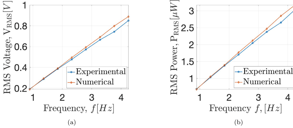
Fig. 7. Prototype performance considering one triboelectric unit (conductor-electrode-conductor): Experimental and numerical response of the triboelectric unit under varying excitation frequency for the (a) RMS voltage and (b) RMS power.
