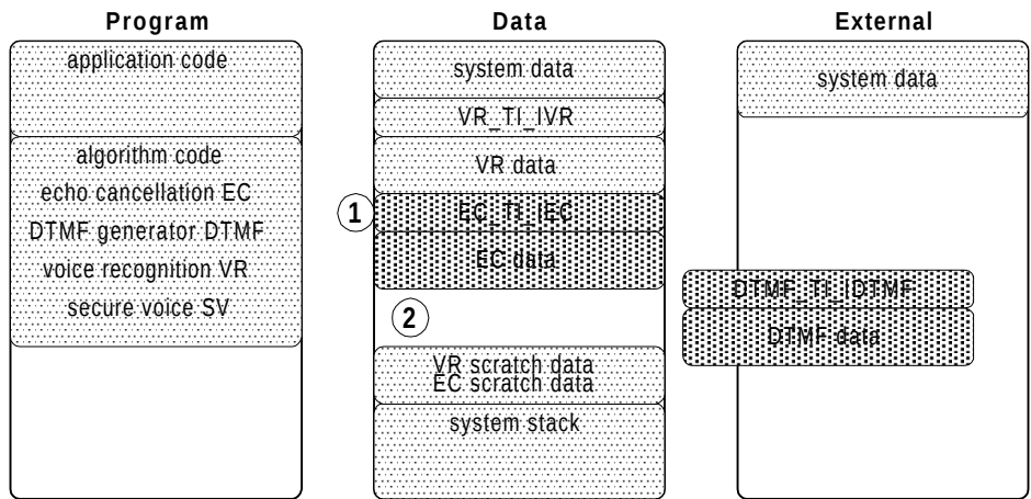
Figure 10. Algorithm Can Not Be Created
