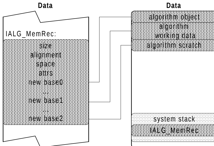
Figure 6b. After Move, Memory Descriptor Points to New Location
