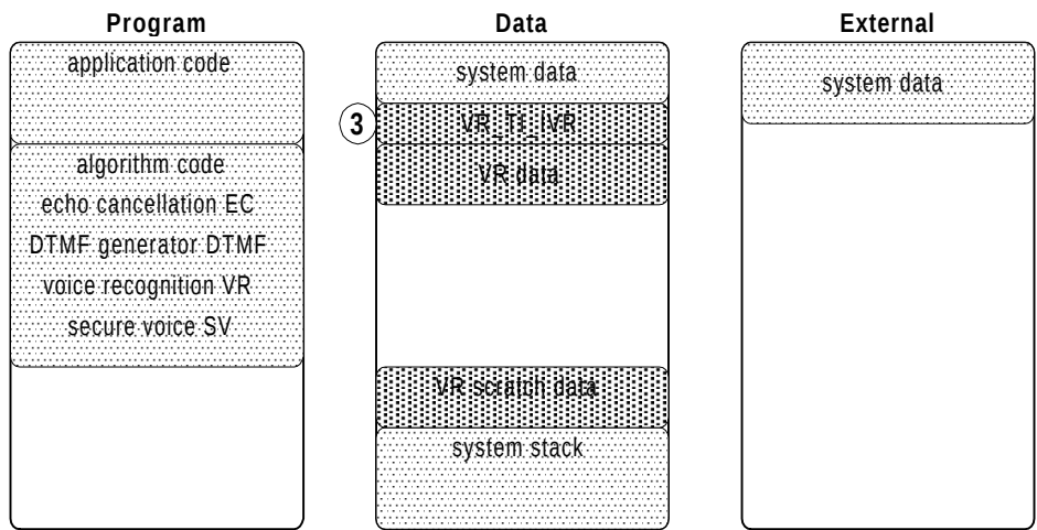
Figure 9. Algorithm Instance Data
