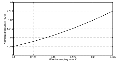
Fig. 3. Normalized frequency versus effective coupling factor
