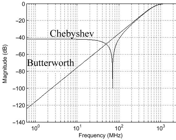
Fig. 10. Theoretical NTF of 1-bit second-order \Sigma\Delta with Butterworth and inverse Chebyshev structures.
