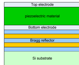
Fig. 1. Solid mounted resonator schematic cross section
