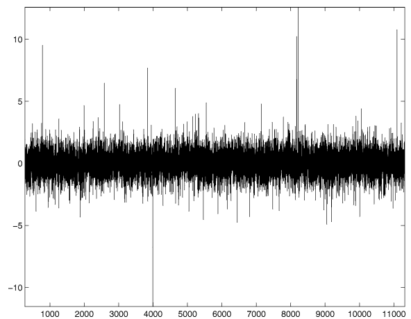
Fig. 3. Signal s_{\text{steps}}(n) .
