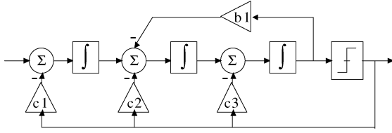
Fig. 9. \Sigma\Delta feedback structure with optional local feedback.
