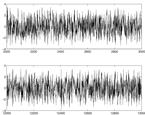
Fig. 5. Signal s_{\text{circle}}(n) .
