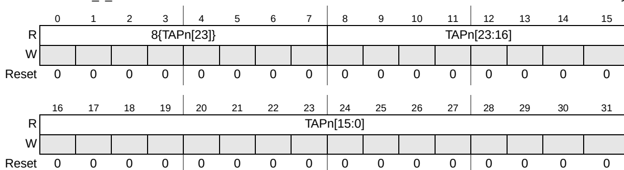
Figure 28-9. Decimation Filter TAPn Register (DECFLT_x_TAPn)
