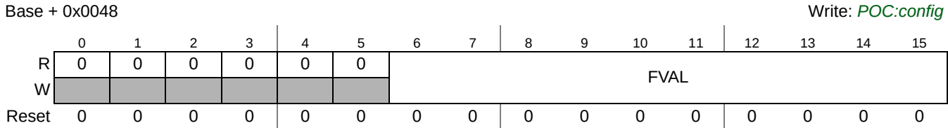
Figure 22-35. Sync Frame ID Acceptance Filter Value Register (SFIDAFVR)
