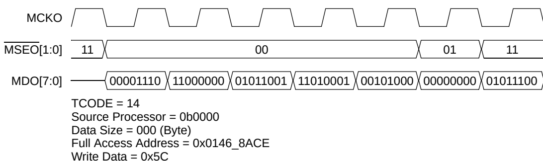
Figure 31-35. Data Trace—Data Read with Sync Message
