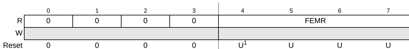
Figure 17-6. Flash ECC Master Number (ECSM_FEMR) Register
