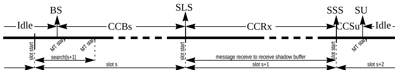
Figure 22-129. Message Reception Timing
