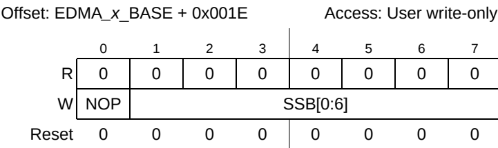
Figure 21-15. eDMA Set START Bit Register (EDMA_x_SSBR)
