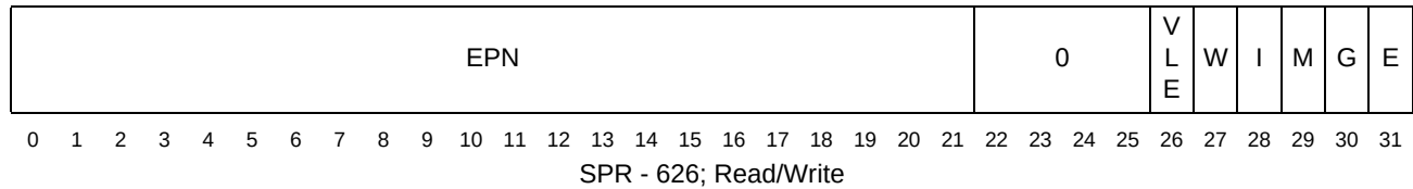
Figure 33-4. MMU Assist Register 2 (MAS2)
