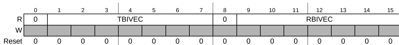
Figure 22-16. Message Buffer Interrupt Vector Register (MBIVEC)
