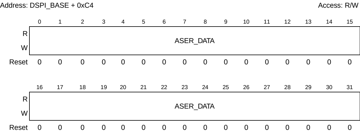
Figure 25-14. DSPI DSI Alternate Serialization Data Register (DSPI_ASDR)
