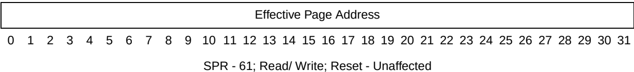
Figure 13-5. DEAR
