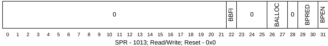
Figure 33-1. Branch Unit Control & Status Register (BUCSR)
