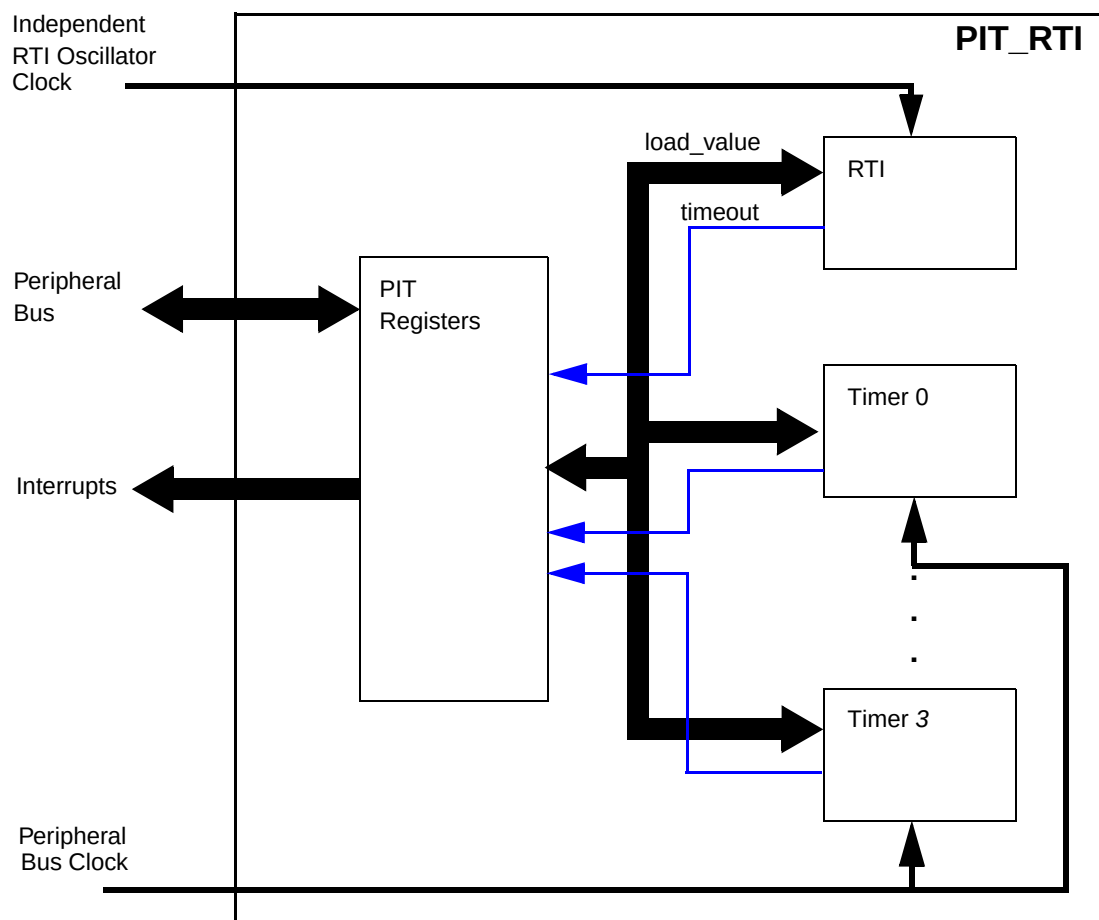
Figure 20-1. Block diagram of PIT_RTI
