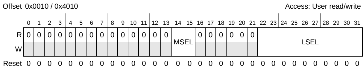
Figure 12-7. FLASH_x_LMSR Register
