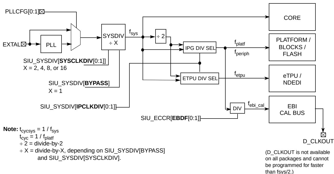
Figure 6-1. PXR40 Block Operating Frequency Domain Diagram
