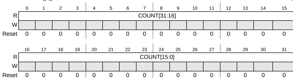
Figure 28-12. Decimation Filter Final Integration Count Value Register (DECFLT_x_FINTCNT)
