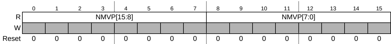
Figure 22-37. Network Management Vector Registers (NMVR0–NMVR5)
