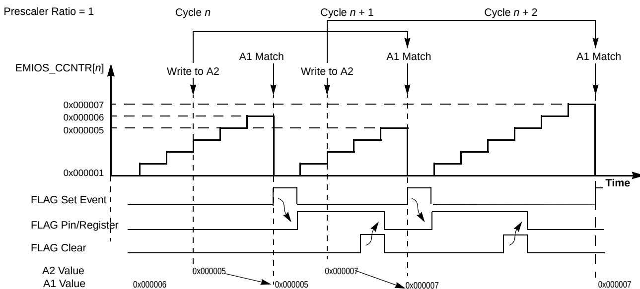
Figure 23-34. Modulus Counter Buffered (MCB) Up Count Mode
