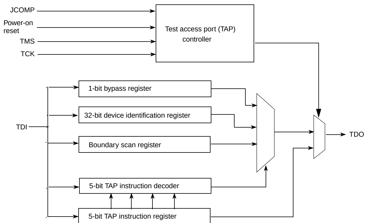
Figure 32-1. JTAG Controller Block Diagram
