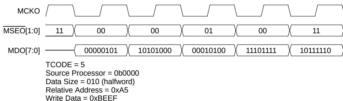
Figure 31-34. Data Trace—Data Write Message
