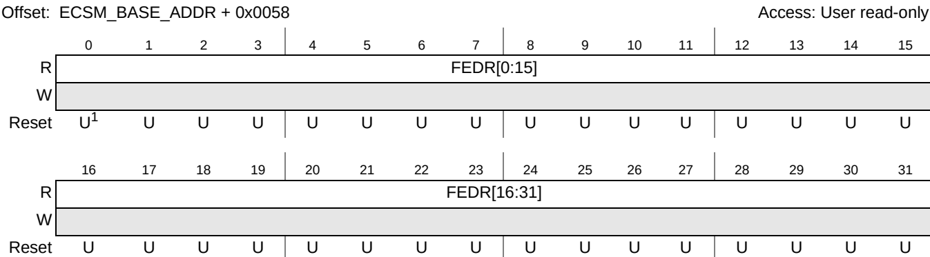
Figure 17-8. Flash ECC Data High (ECSM_FEDRH) Register
