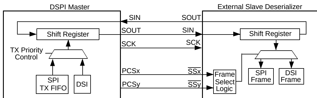
Figure 25-24. Example of System using DSPI in CSI Configuration
