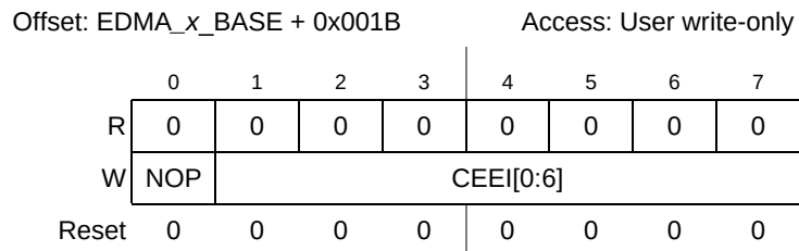
Figure 21-12. eDMA Clear Enable Error Interrupt Register (EDMA_x_CEEIR)
