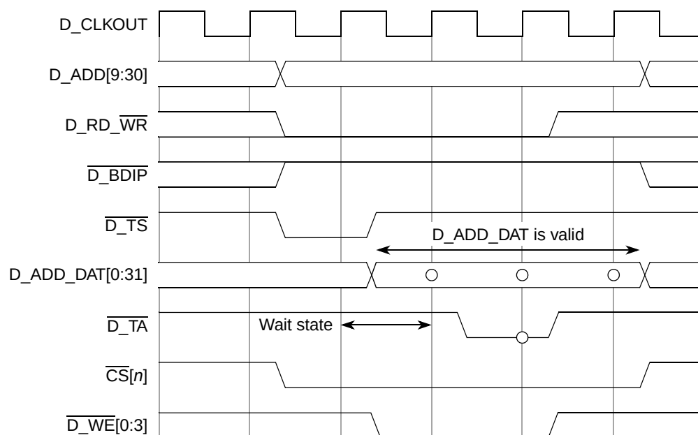
Figure 30-15. Single Beat 32-bit Write Cycle, \overline{\text{CS}} Access, One Wait State
