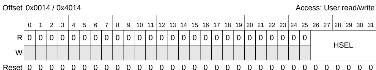
Figure 12-8. FLASH_x_HSR Register
