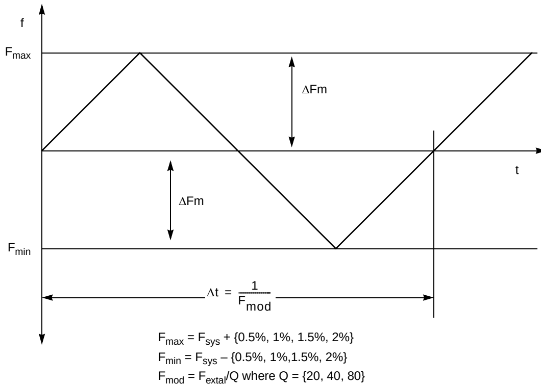
Figure 6-8. Frequency Modulation Waveform
