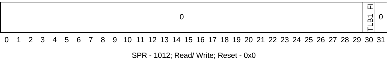
Figure 13-6. MMU Control and Status Register 0 (MMUCSR0)
