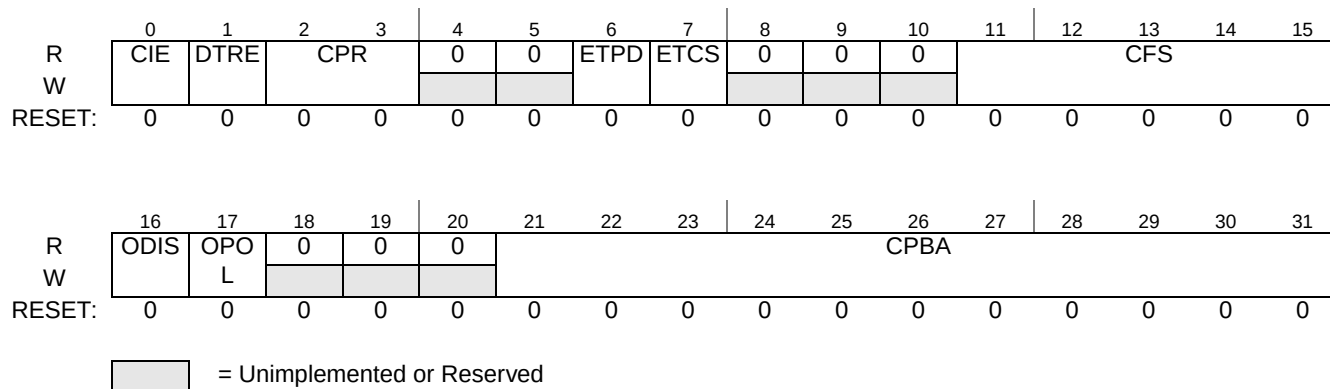
Figure 29-23. ETPUCxCR Register
