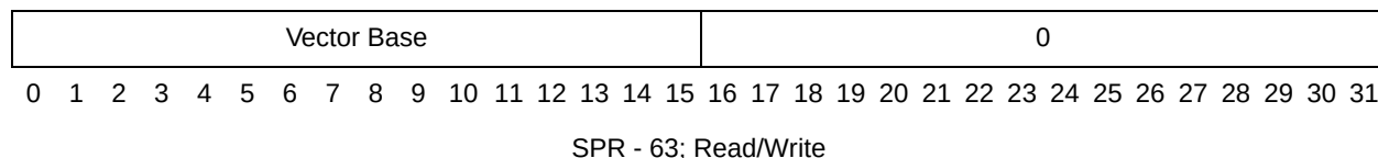
Figure 13-15. PXR40 Interrupt Vector Prefix Register (IVPR)
