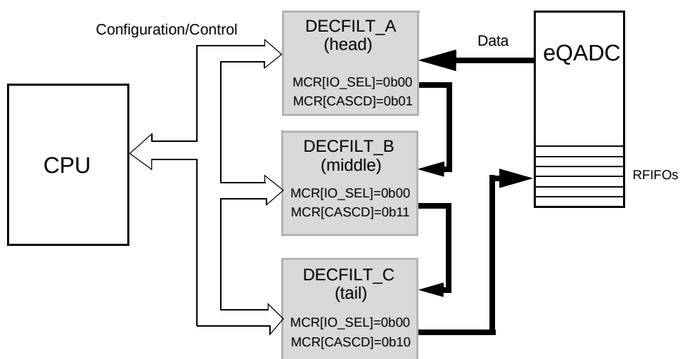
Figure 28-18. Cascaded Filters
