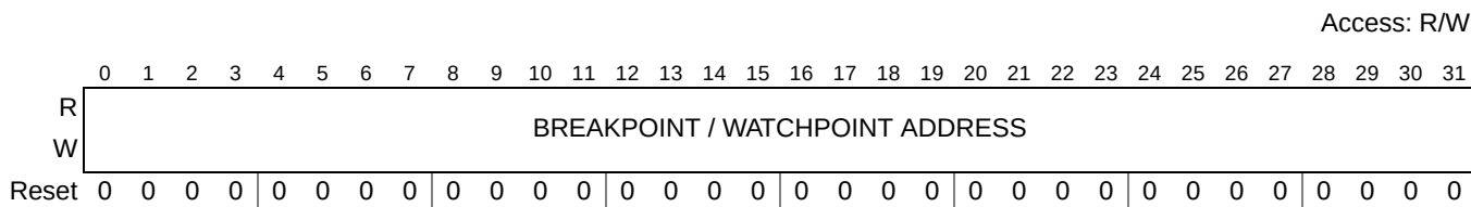
Figure 31-51. Breakpoint / Watchpoint Address Registers (BWA1, BWA2)
