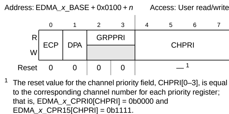
Figure 21-23. eDMA Channel n Priority Register ( EDMA_x_CPRn )
