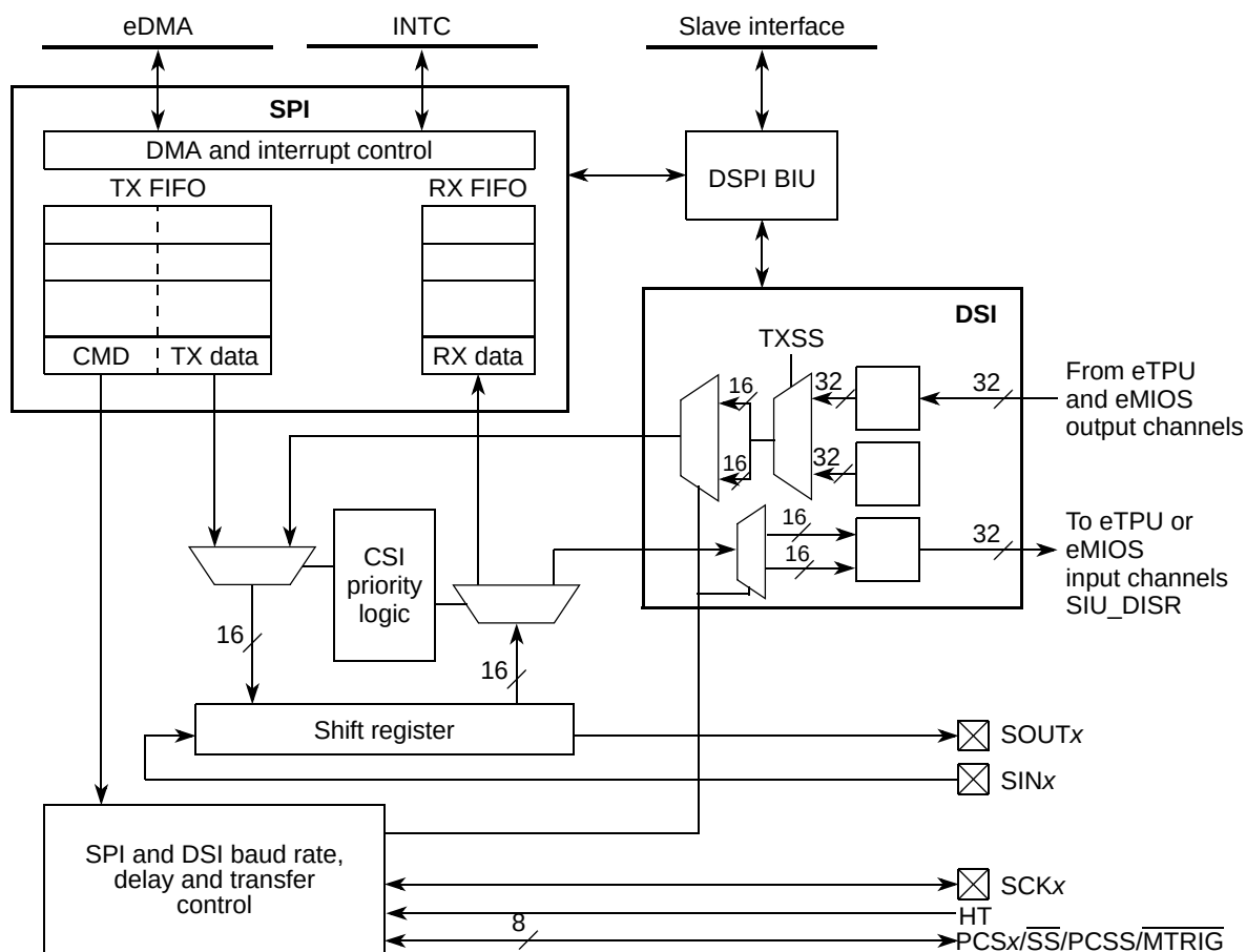
Figure 25-1. DSPI Block Diagram
