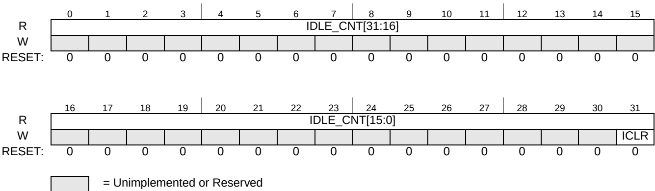
Figure 29-13. ETPUIDLER Register
