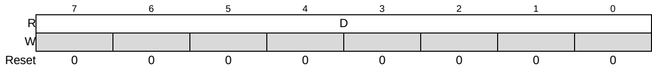
Figure 26-12. LIN Receive Register (eSCI_LRR)
