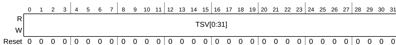
Figure 20-3. Timer Load Value Register (PIT_RTI_LDVAL, PIT_CHn_LDVAL)
