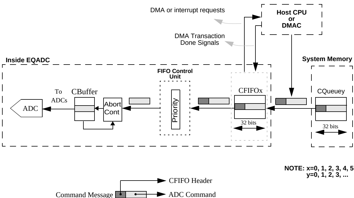
Figure 27-42. Command Flow during EQADC operation
