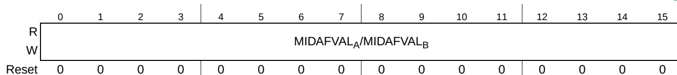
Figure 22-60. Receive FIFO Message ID Acceptance Filter Value Register (RFMIDAFVR)
