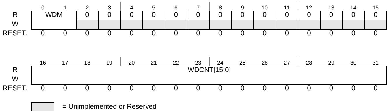
Figure 29-12. ETPUWDTR Register
