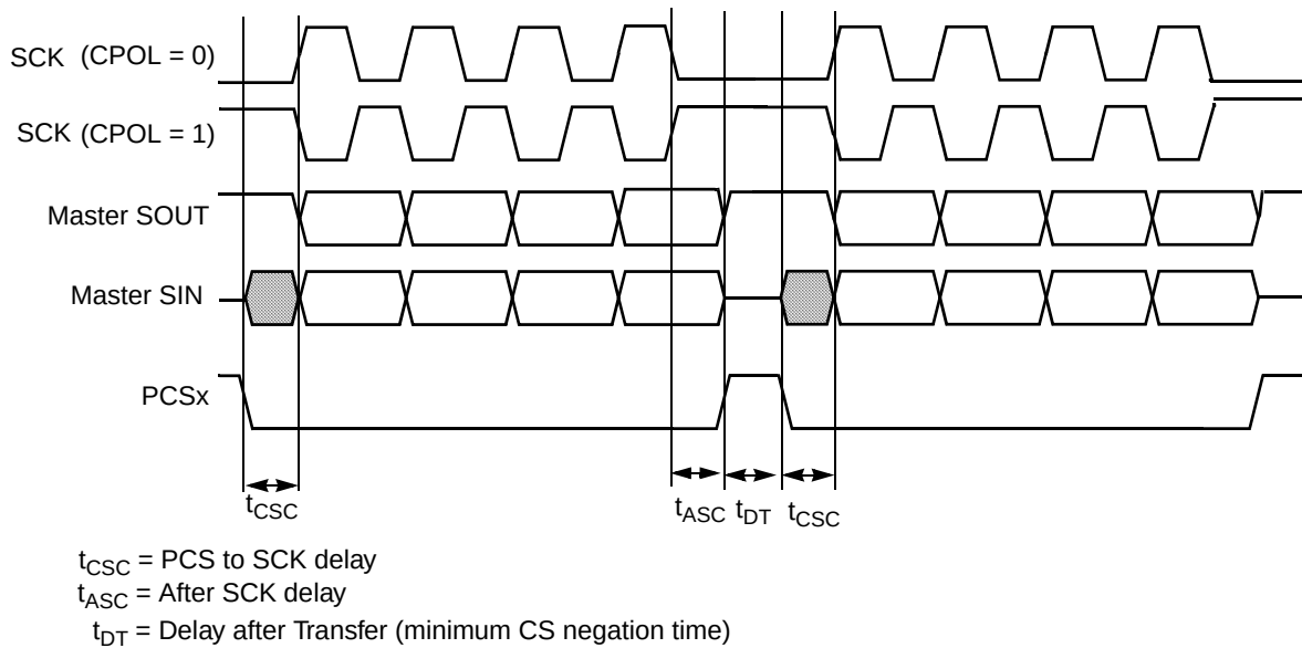
Figure 25-33. Example of Non-Continuous Format (CPHA=1, CONT=0)
