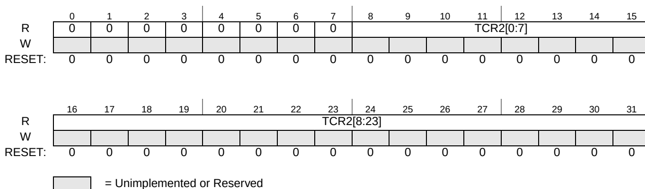
Figure 29-10. ETPUTB2R Register
