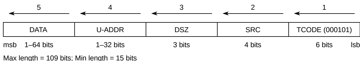
Figure 31-30. Data Write Message Format
