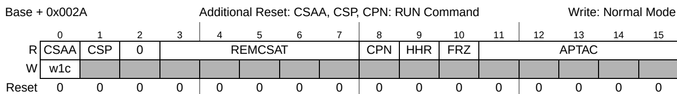
Figure 22-20. Protocol Status Register 1 (PSR1)
