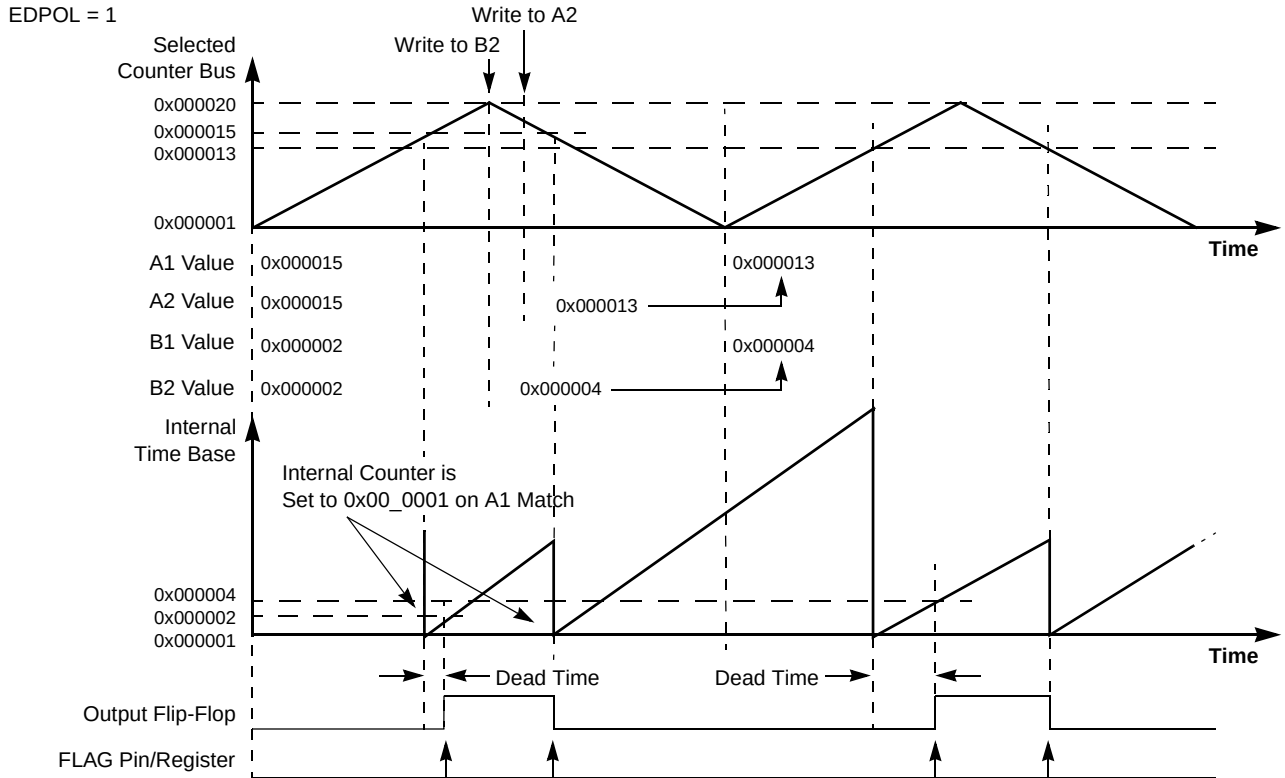
Figure 23-48. OPWMCB with Leading Dead Time Insertion
