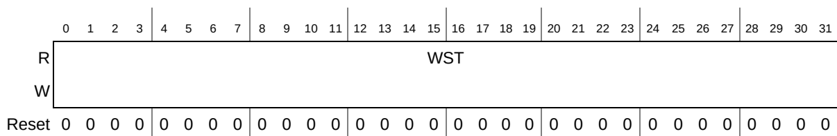
Figure 18-4. SWT Window Register (SWT_WN)
