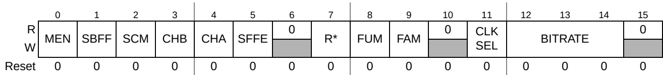
Figure 22-3. Module Configuration Register (MCR)
