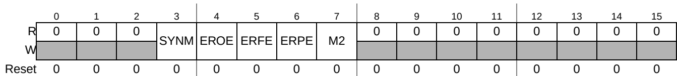
Figure 26-14. Control Register 3 (eSCI_CR3)
