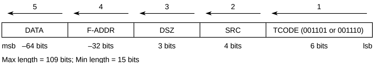
Figure 31-33. Data Write/Read with Sync. Message Format
