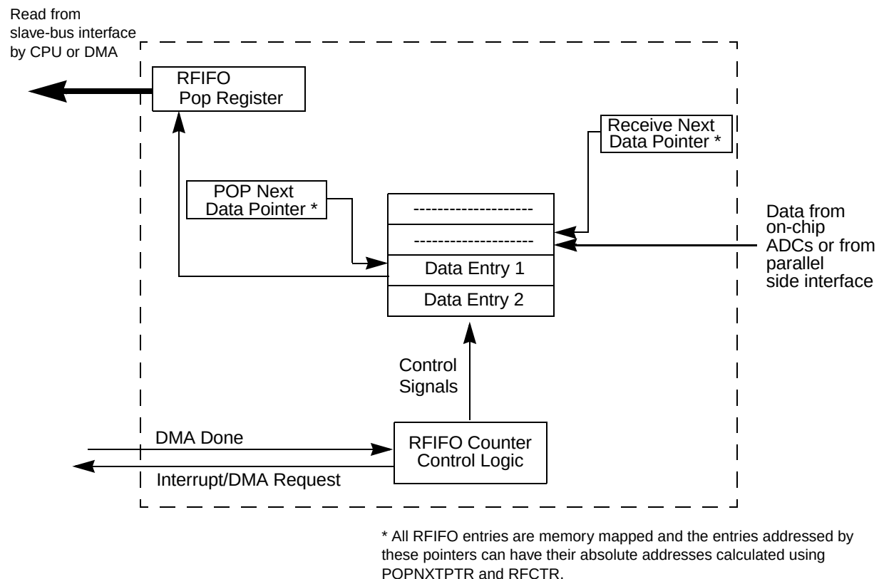
Figure 27-60. RFIFO Diagram
