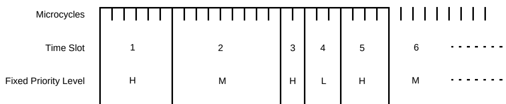
Figure 29-30. Time-Slot Variation
