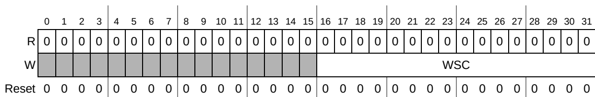
Figure 18-5. SWT Service Register (SWT_SR)
