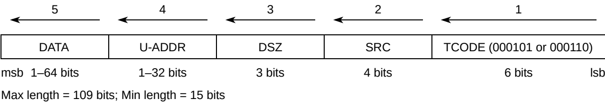
Figure 31-54. Data Write/Read Message Format
