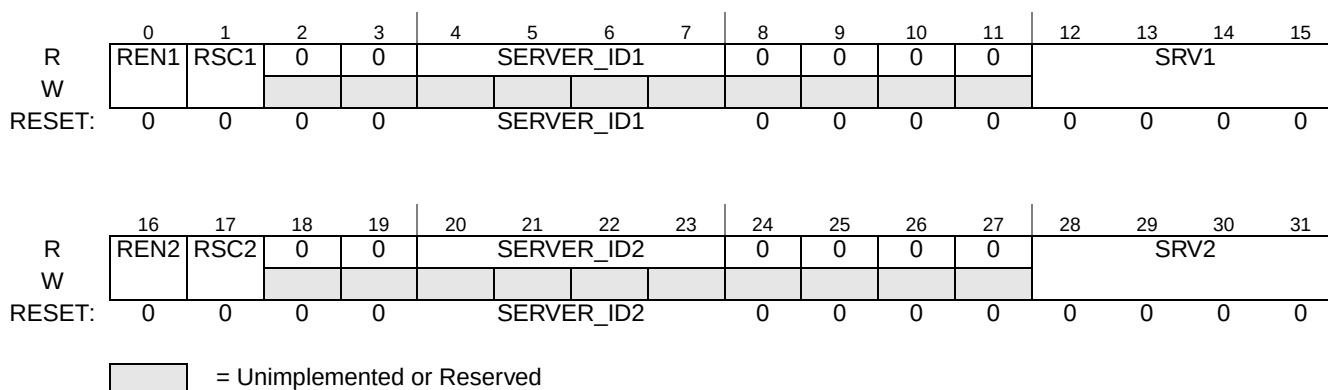
Figure 29-11. ETPUREDCCR Register
