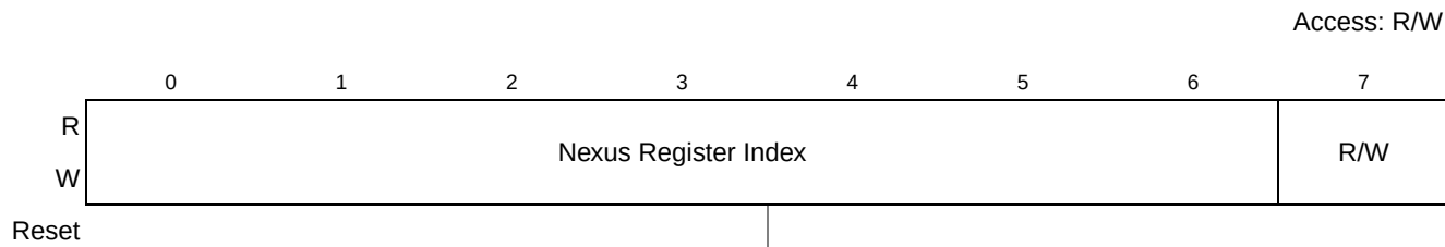
Figure 31-53. JTAG DR for NEXUS Register Access
