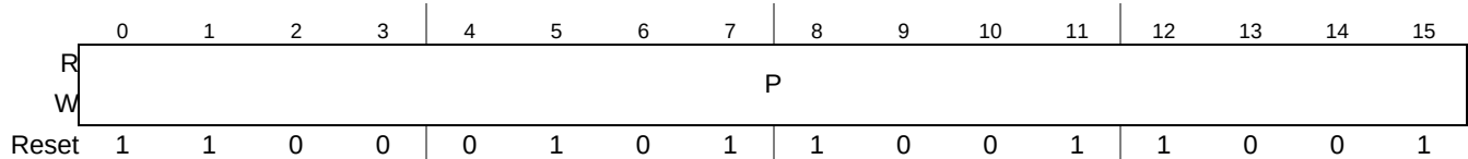
Figure 26-13. LIN CRC Polynomial Register (eSCI_LPR)
