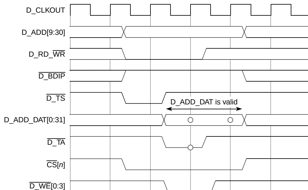
Figure 30-14. Single Beat 32-bit Write Cycle, \overline{\text{CS}} Access, Zero Wait States
