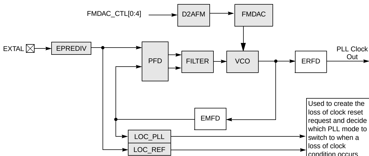
Figure 6-2. FMPLL Block Diagram
