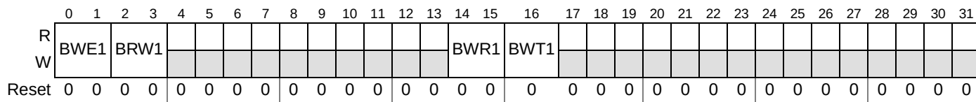
Figure 31-49. Break / Watchpoint Control Register 1 (BWC1)
