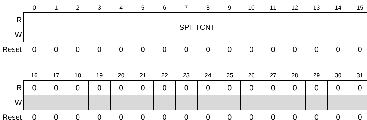
Figure 25-4. DSPI Transfer Count Register (DSPI_TCR)
