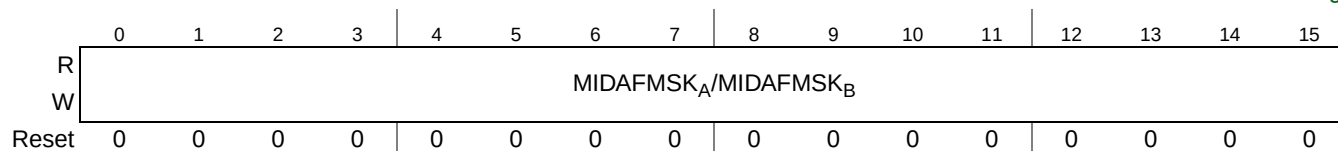
Figure 22-61. Receive FIFO Message ID Acceptance Filter Mask Register (RFMIAFMR)
