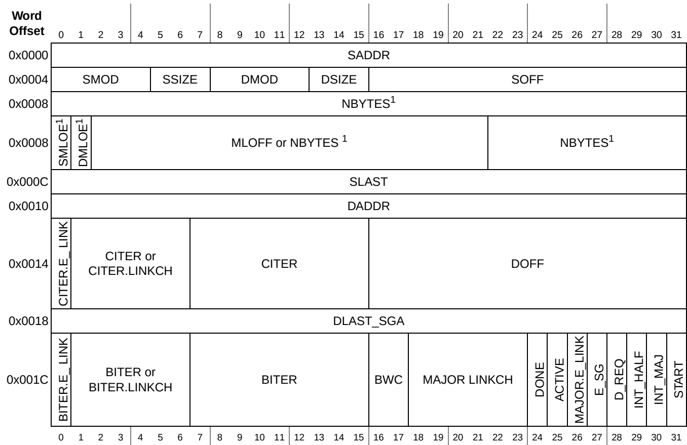
Figure 21-24. TCD Structure
