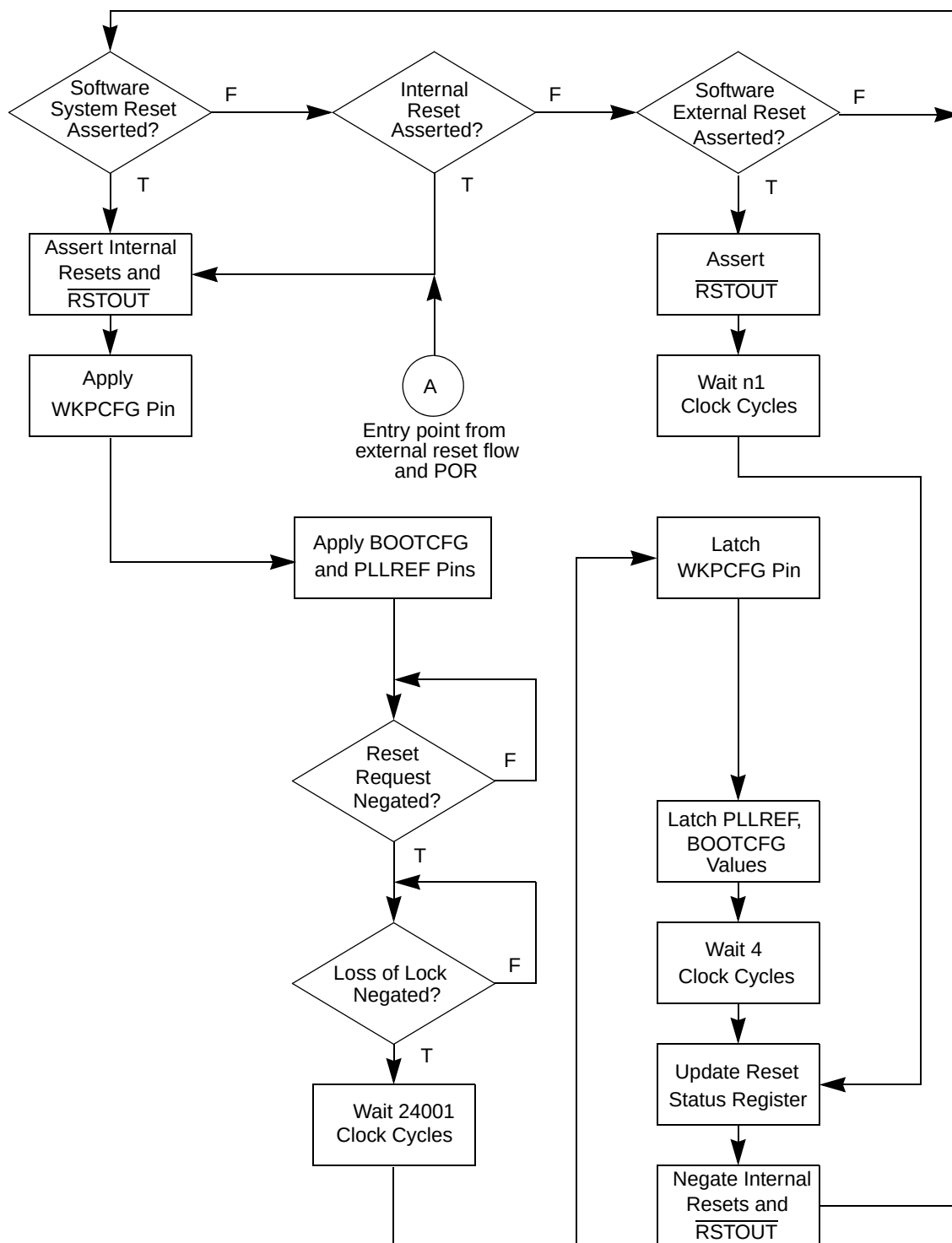
Figure 4-2. Internal Reset Flow Diagram
