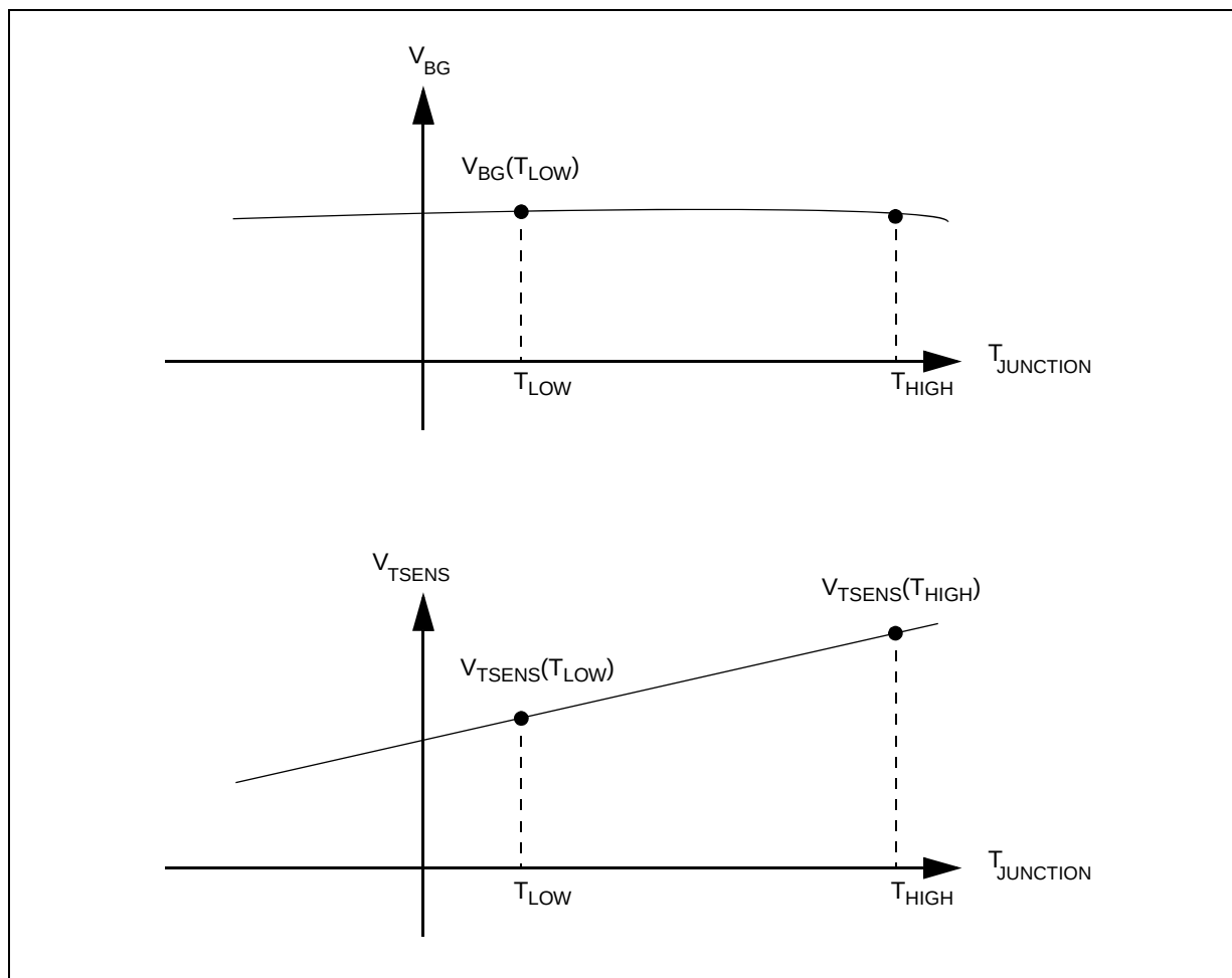
Figure 34-1. Calibration Points
