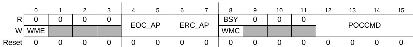
Figure 22-9. Protocol Operation Control Register (POCR)
