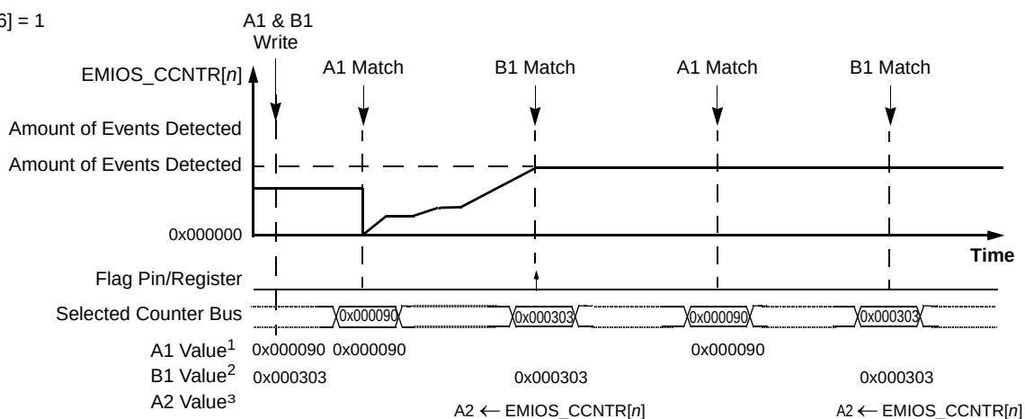
Figure 23-27. PEC Continuous Mode Example
