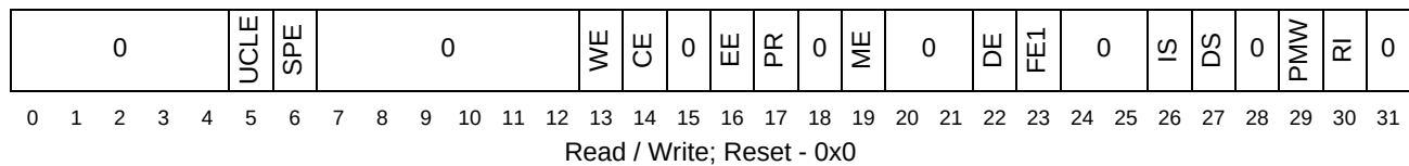
Figure 33-6. Machine State Register (MSR)
