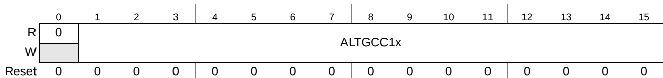
Figure 27-39. ADC0/1 Alternate x Gain Register (ADC0/1_AGRx, x=1-2)
