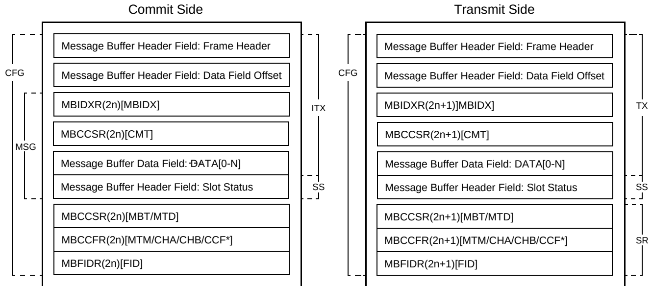
Figure 22-131. Double Transmit Message Buffer Access Regions Layout
