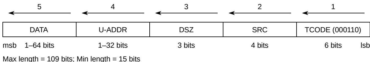
Figure 31-32. Error Message Format
