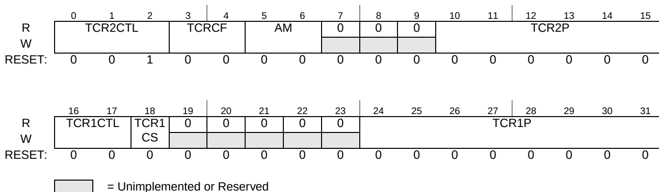
Figure 29-8. ETPUTBCR Register
