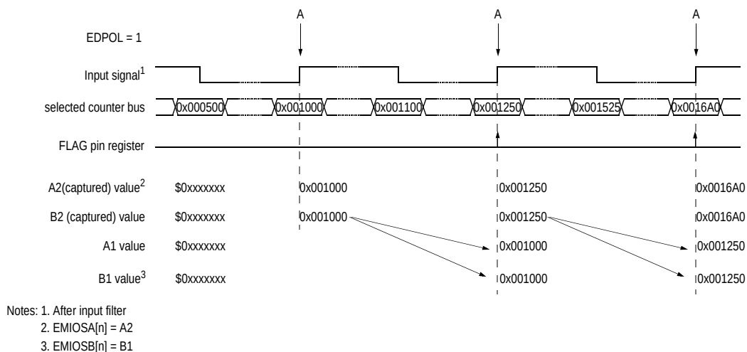
Figure 23-20. IPM Example
