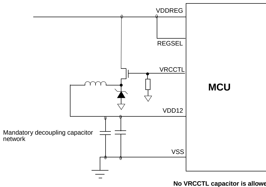
Figure 5-11. VRC 1.2V buck SMPS LDO configuration with external MOS - Schottky diode
