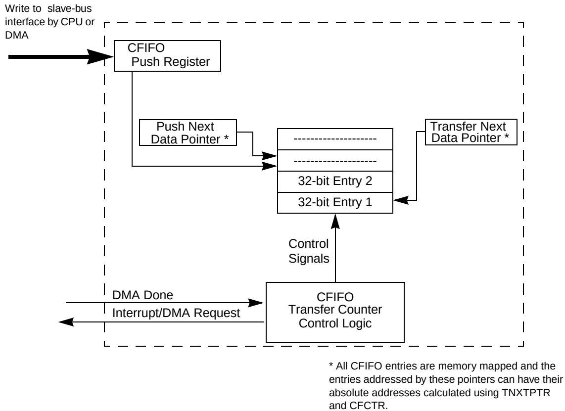
Figure 27-49. CFIFO Diagram
