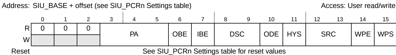
Figure 7-14. Pad Configuration Register (SIU_PCRn)
