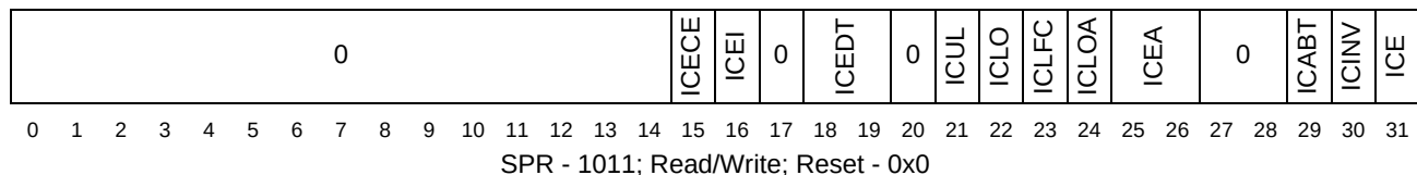
Figure 33-2. L1 Cache Control & status Register 1 (L1CSR1)
