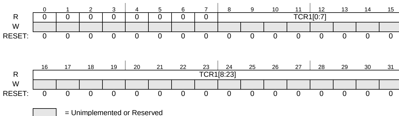
Figure 29-9. ETPUTB1R Register
