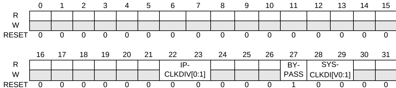
Figure 7-25. System Clock Register (SIU_SYSDIV)
