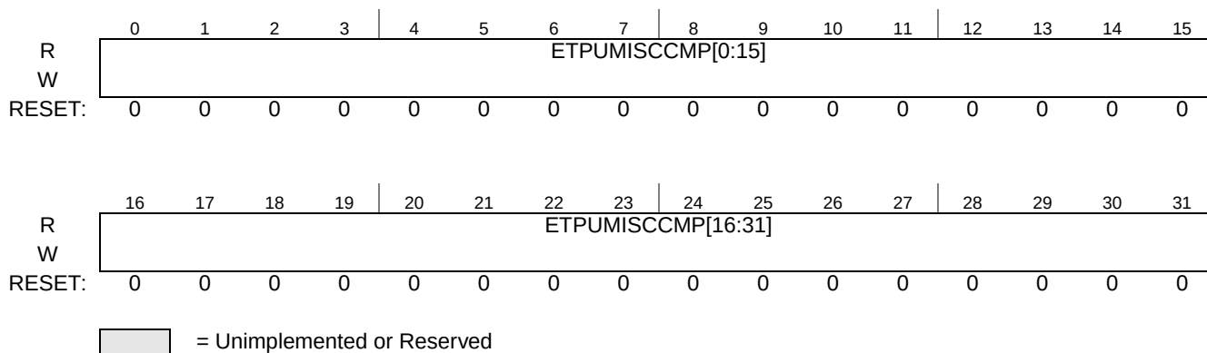
Figure 29-5. ETPUMISCCMPR Register
