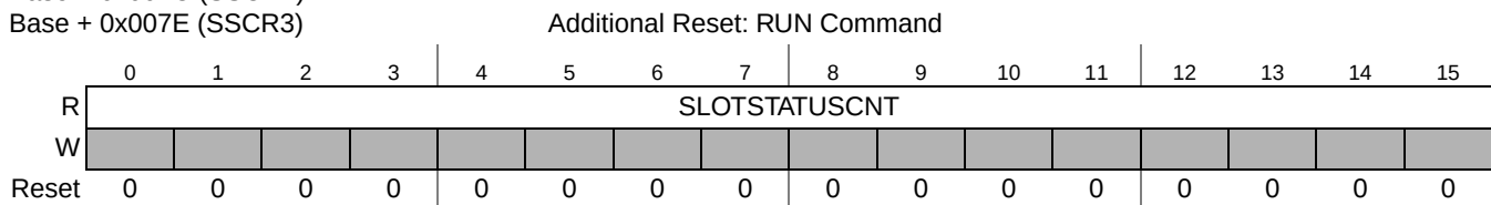
Figure 22-47. Slot Status Counter Registers (SSCR0–SSCR3)
