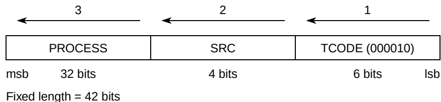
Figure 31-14. Ownership Trace Message Format
