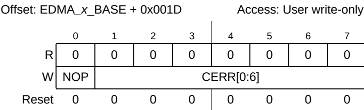
Figure 21-14. eDMA Clear Error Register (EDMA_x_CER)
