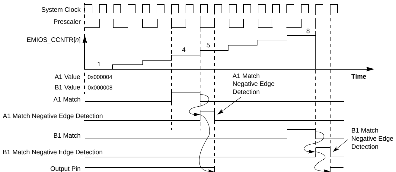
Figure 23-40. OPWFMB A1 and B1 Match to Output Register Delay
