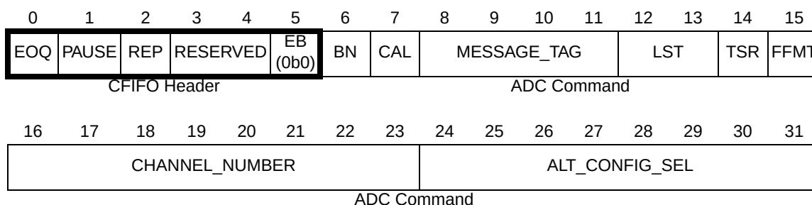
Figure 27-44. Conversion Command Format for Alternate Configurations
