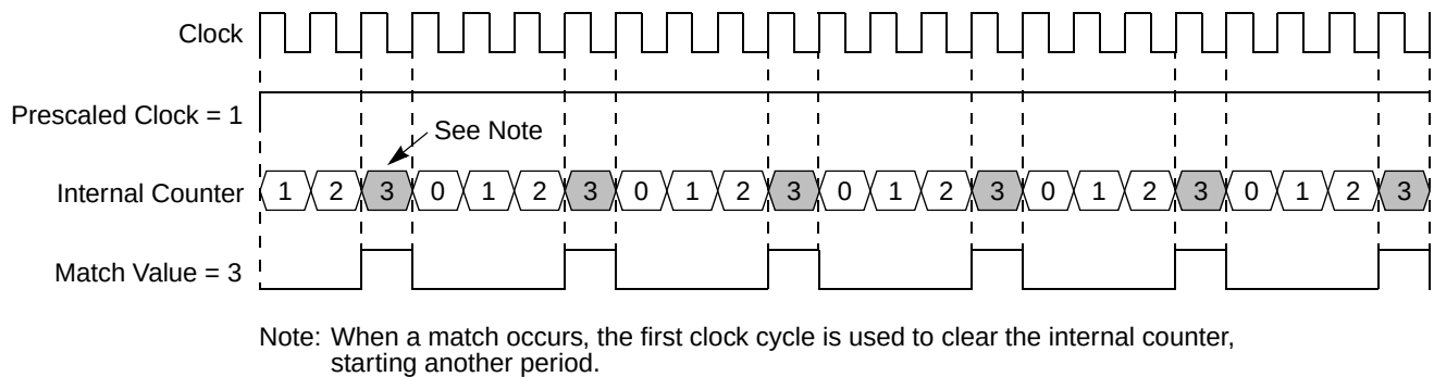
Figure 23-61. Time Base Period when Running in the Fastest Prescaler Ratio
