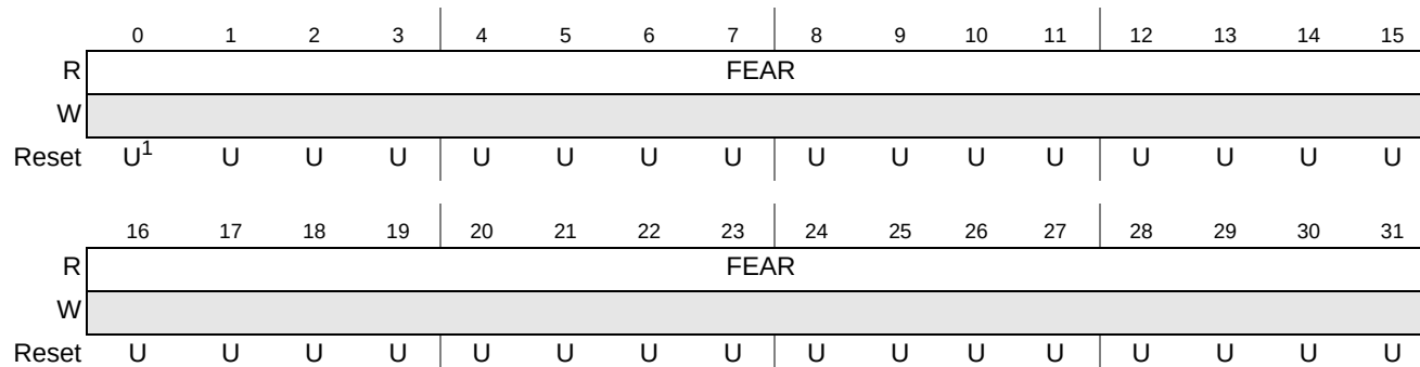
Figure 17-5. Flash ECC Address (ECSM_FEAR) Register
