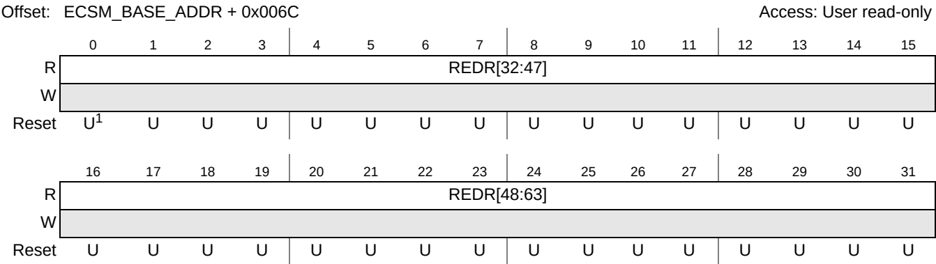
Figure 17-15. RAM ECC Data Low (ECSM_REDRL) Register
