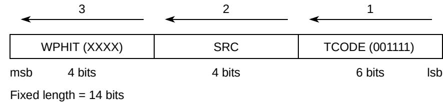
Figure 31-57. Watchpoint Message Format
