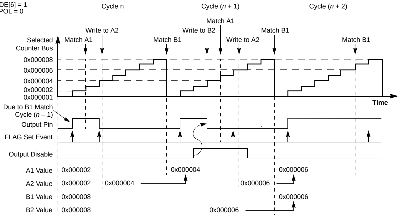
Figure 23-55. OPWMB Mode with Active Output Disable
