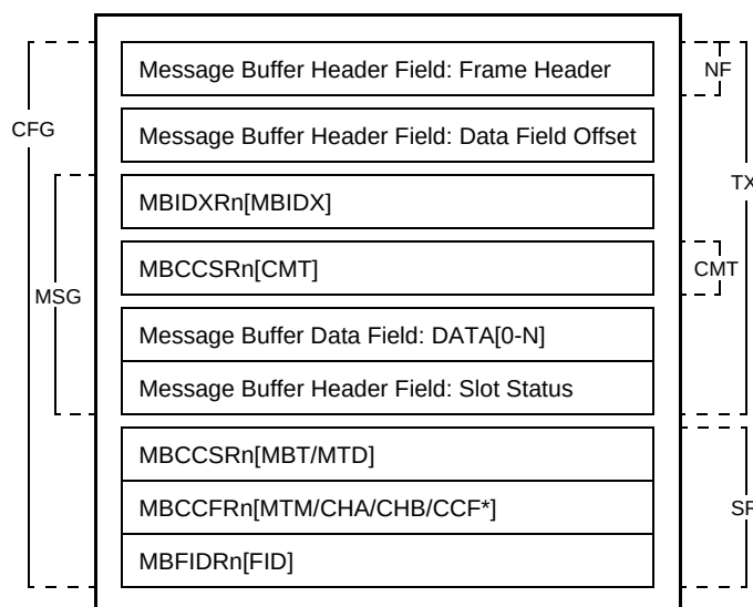
Figure 22-119. Single Transmit Message Buffer Access Regions
