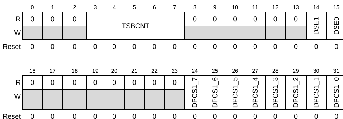
Figure 25-17. DSPI DSI Configuration Register 1 (DSPI_DSICR1)
