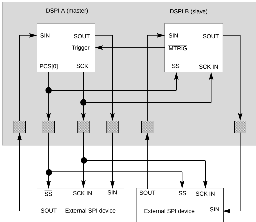
Figure 7-53. DSPI Parallel Chaining
