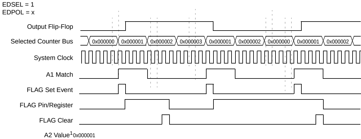
Figure 23-17. SAOC Example with Flag Behavior
