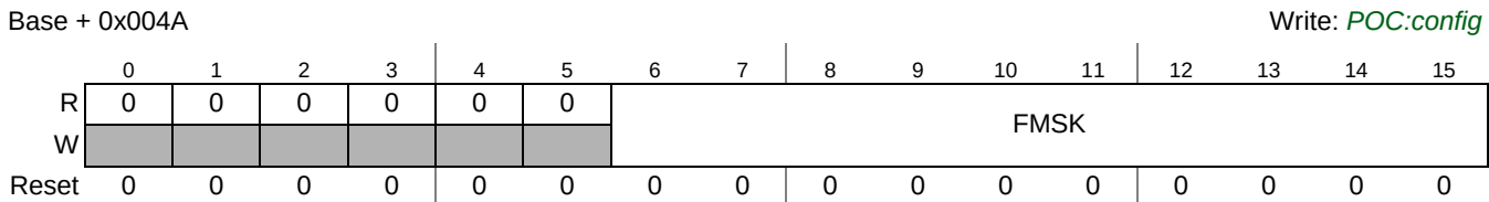
Figure 22-36. Sync Frame ID Acceptance Filter Mask Register (SFIDAFMR)
