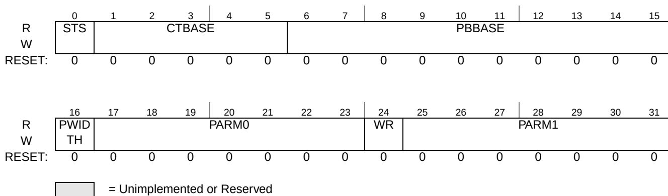
Figure 29-4. ETPUCDCR Register
