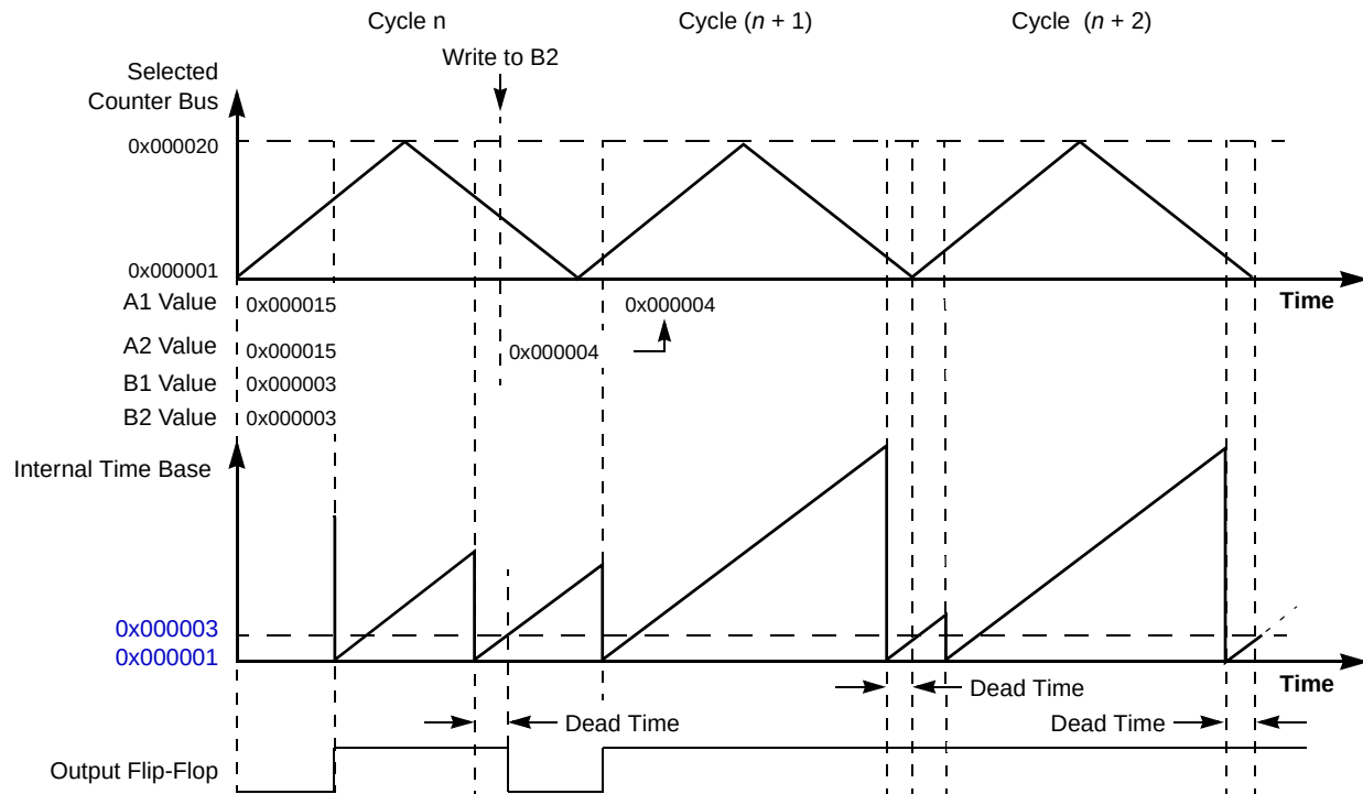
Figure 23-50. OPWMCB with 100% Duty Cycle (A1 = 4 and B1 = 3)
