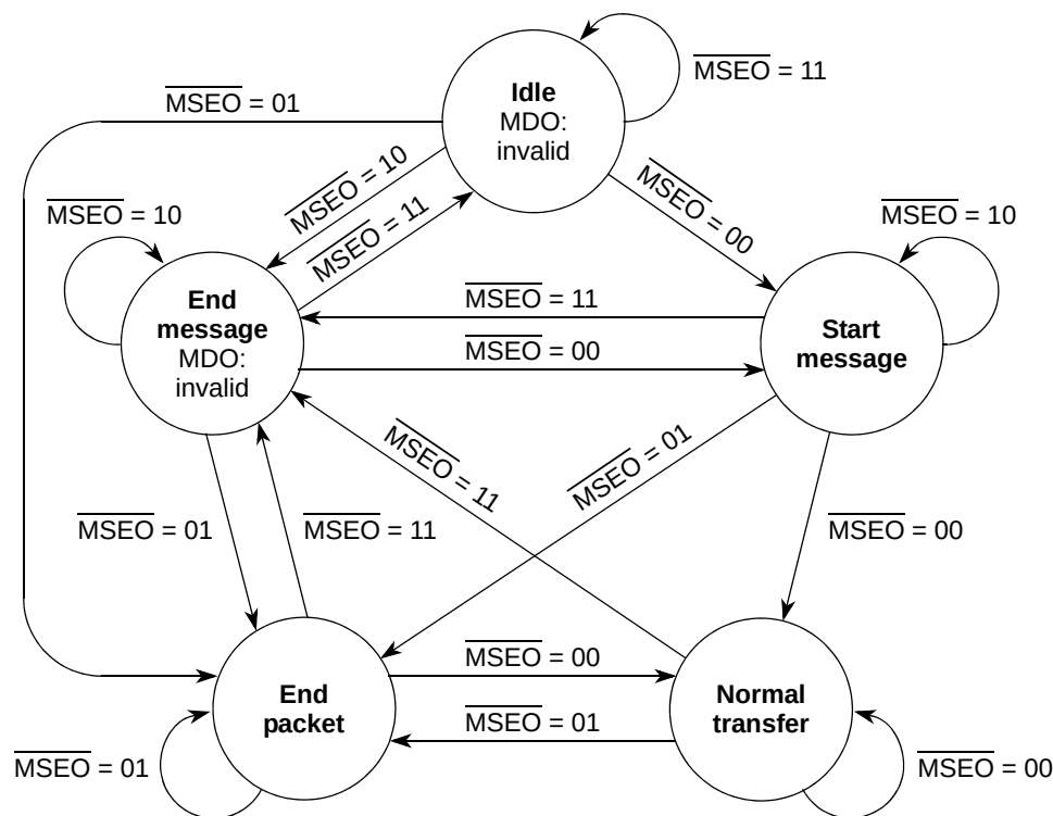
Figure 31-5. MSEO Transfers
