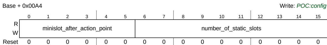
Figure 22-70. Protocol Configuration Register 2 (PCR2)
