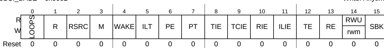
Figure 26-3. Control Register 1 (eSCI_CR1)
