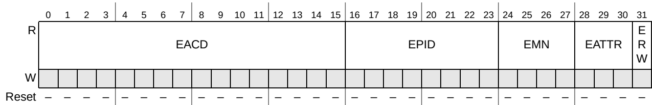
Figure 16-4. MPU Error Detail Register, MPU Port n (MPU_EDR n )
