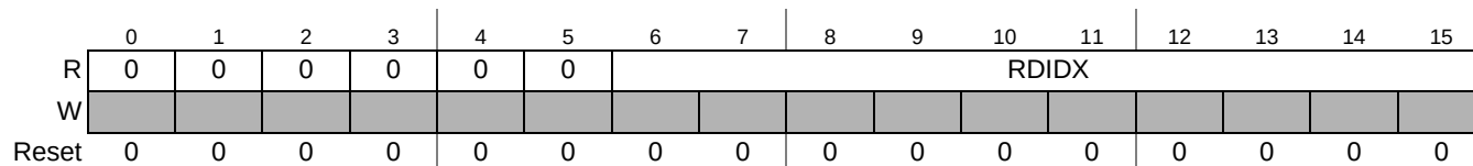
Figure 22-57. Receive FIFO A Read Index Register (RFARIR)
