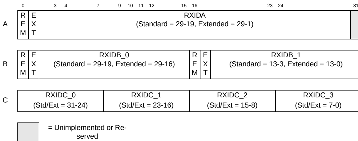
Figure 24-4. ID Table 0 - 7
