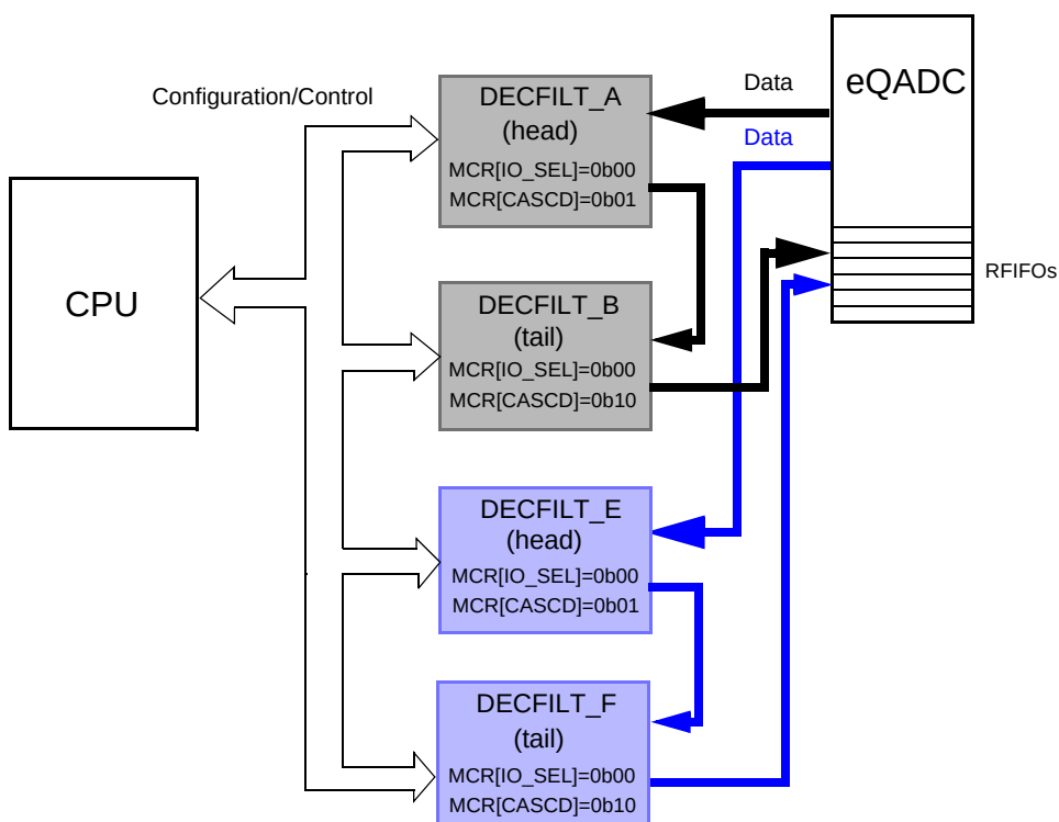
Figure 28-19. Multiple Cascaded Filters
