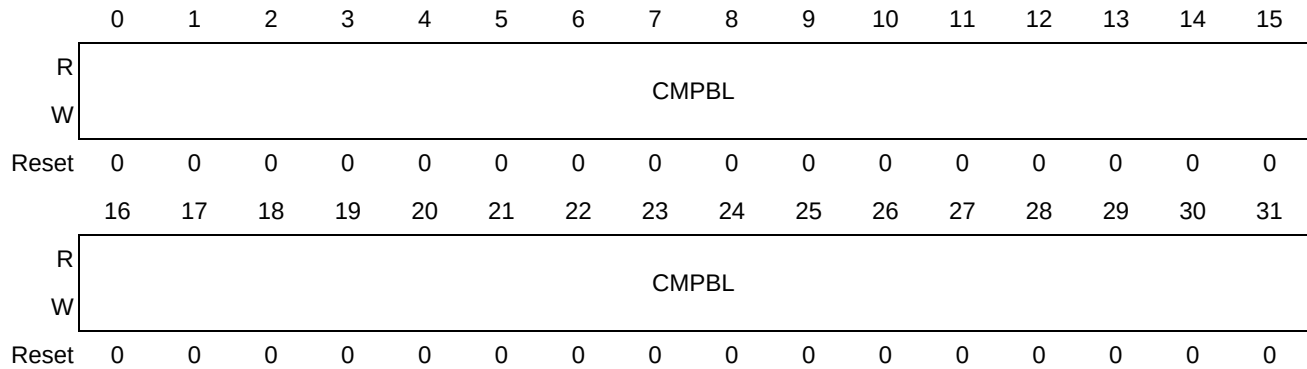
Figure 7-24. Compare B Register Low (SIU_CBRL)
