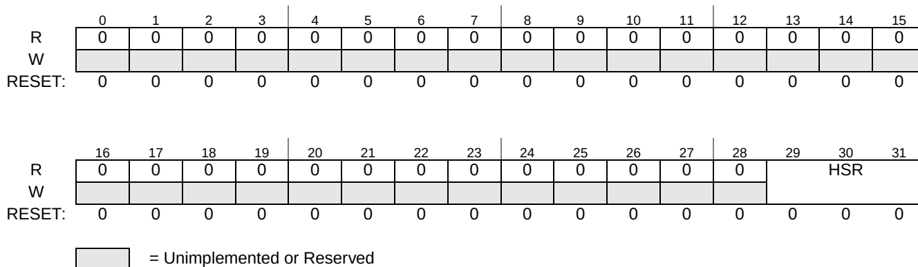
Figure 29-25. ETPUCxHSRR Register
