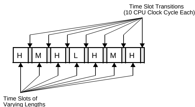
Figure 29-36. Time-Slot Sequence
