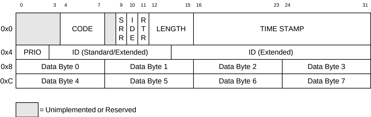
Figure 24-2. Message Buffer Structure
