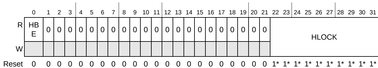
Figure 12-5. FLASH_x_HLR Register
