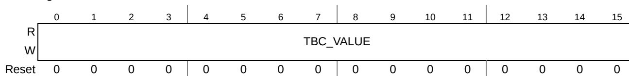
Figure 27-35. ADC Time Base Counter Register (ADC_TBCR)
