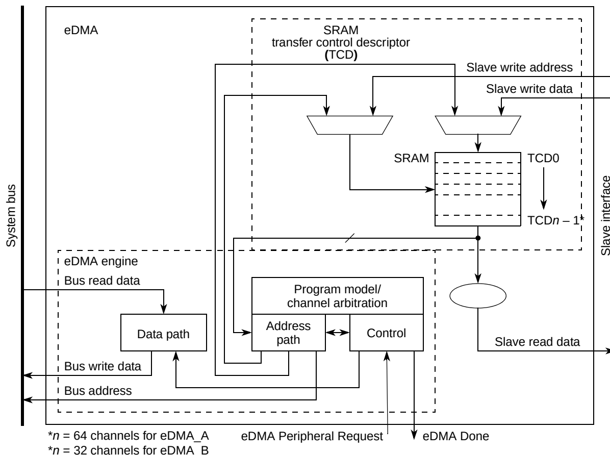
Figure 21-1. eDMA Block Diagram
