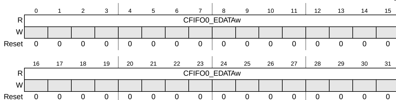
Figure 27-25. EQADC CFIFO0 Extension Registers (EQADC_CF0ERw) (w=0, ..., 3)
