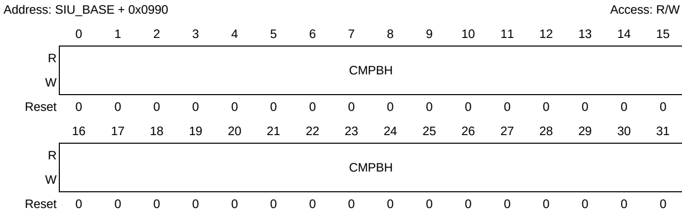
Figure 7-23. Compare B Register High (SIU_CBRH)
