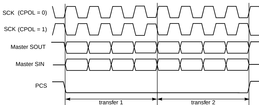
Figure 25-36. Continuous SCK Timing Diagram (CONT=1)
