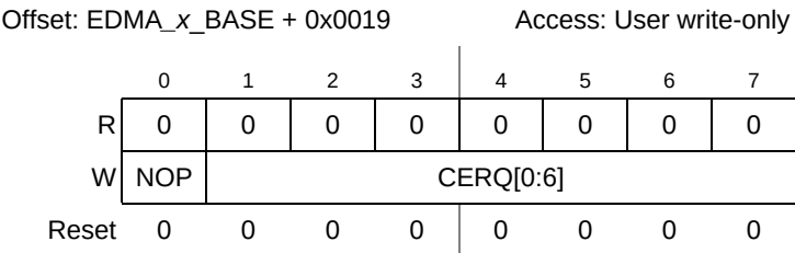
Figure 21-10. eDMA Clear Enable Request Register (EDMA_x_CERQR)
