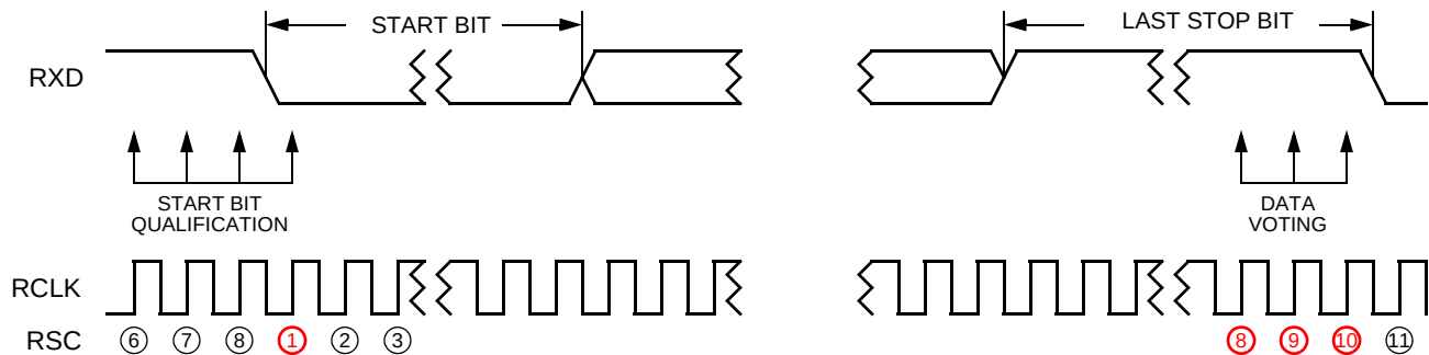
Figure 26-24. Slower Receiver
