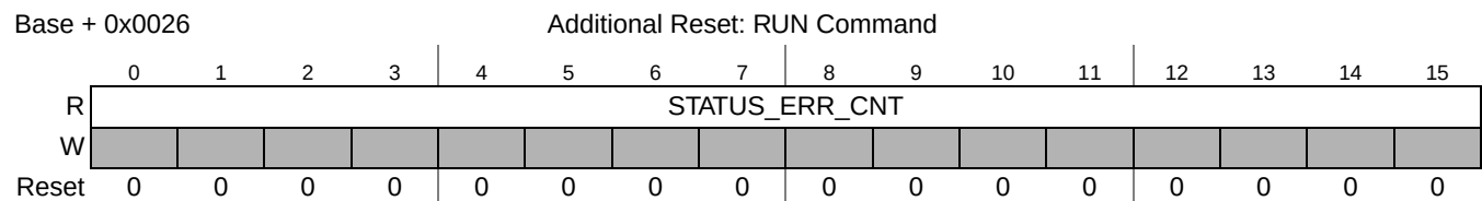
Figure 22-18. Channel B Status Error Counter Register (CBSECR)
