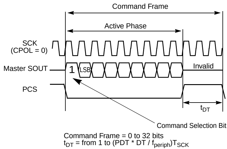
Figure 25-39. Command Frame Format
