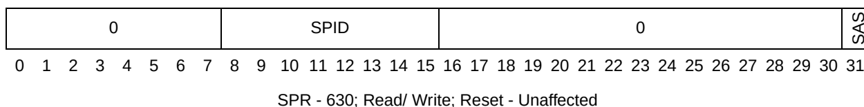
Figure 13-12. MMU Assist Register 6 (MAS6)
