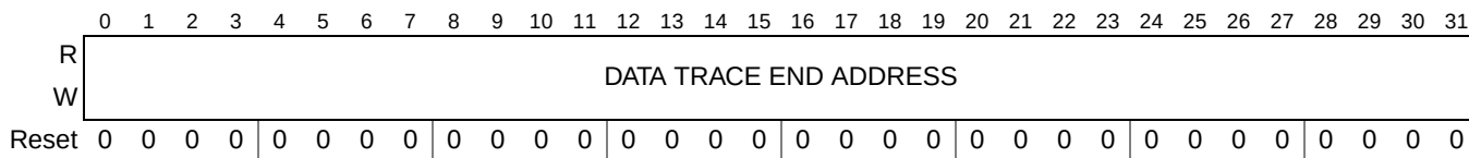
Figure 31-48. Data Trace Start Address Registers (DTEA1, DTEA2)
