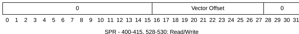
Figure 13-16. PXR40 Interrupt Vector Offset Register (IVOR)
