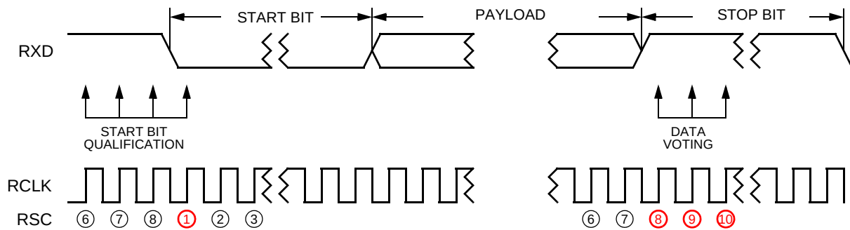
Figure 26-23. Faster Receiver
