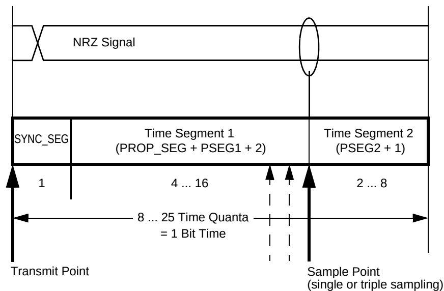
Figure 24-17. Segments within the Bit Time
