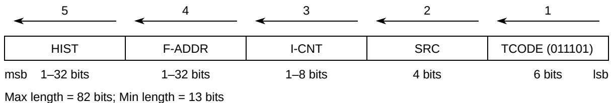
Figure 31-24. Indirect Branch History with Sync. Message Format
