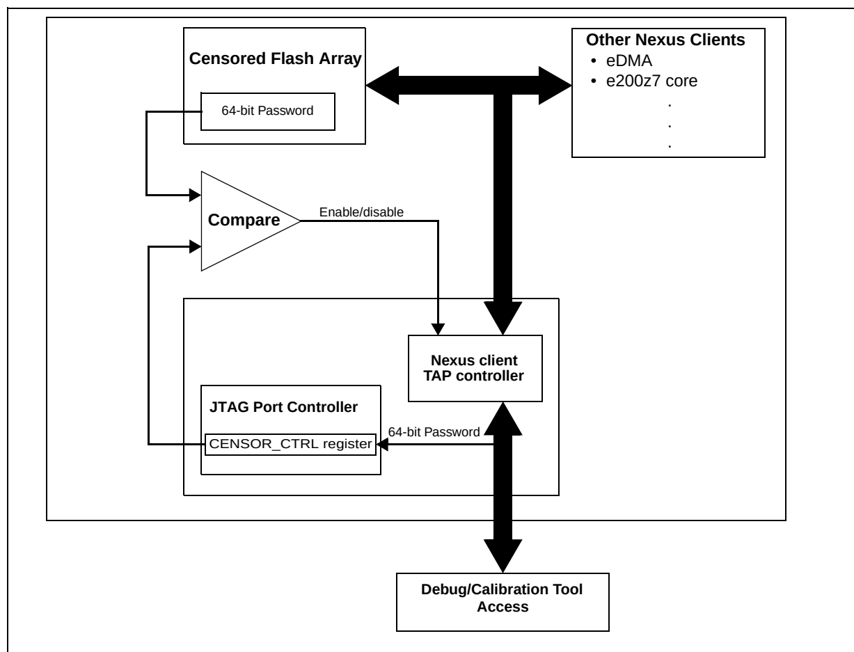
Figure 9-8. Enabling JTAG/Nexus port access on a censored device
