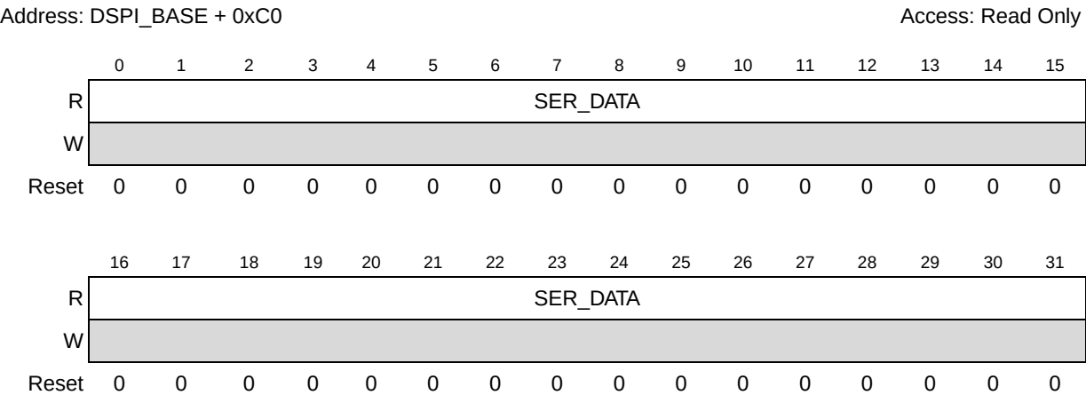
Figure 25-13. DSPI DSI Serialization Data Register (DSPI_SDR)
