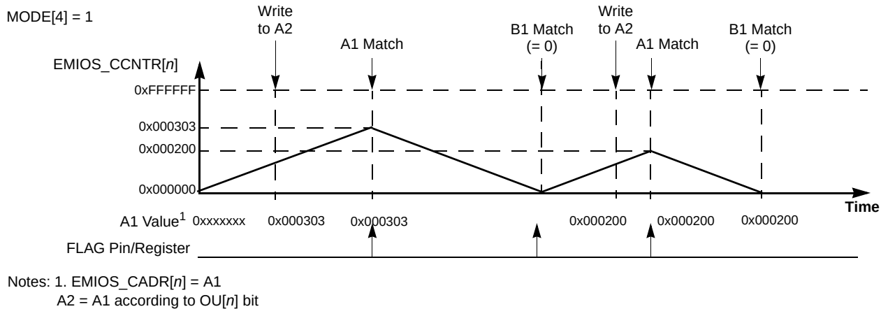
Figure 23-33. MC Up/Down Mode Example
