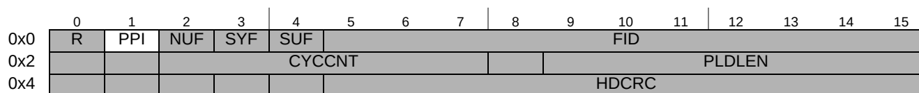
Figure 22-111. Frame Header Structure (Transmit Message Buffer for Key Slot)
