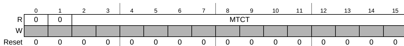
Figure 22-23. Macrotick Counter Register (MTCTR)
