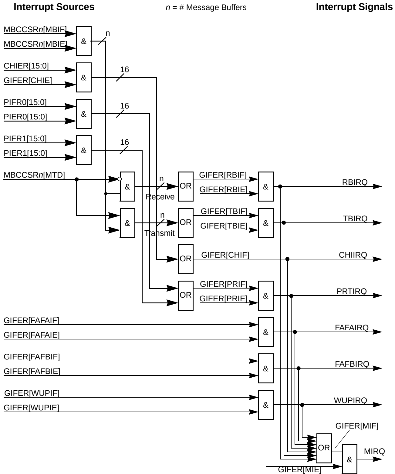
Figure 22-150. Scheme of cascaded interrupt request
