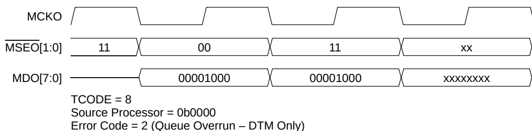
Figure 31-36. Error Message (Data Trace only encoded)
