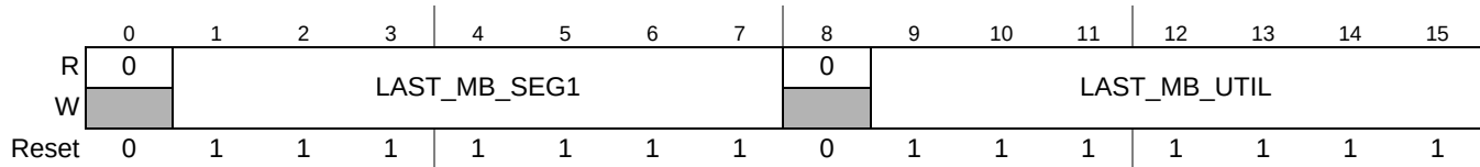
Figure 22-8. Message Buffer Segment Size and Utilization Register (MBSSUTR)
