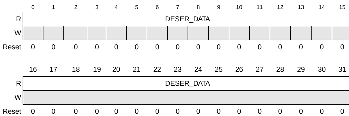
Figure 25-16. DSPI Deserialization Data Register (DSPI_DDR)
