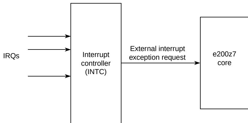
Figure 10-2. INTC Software Vector Mode
