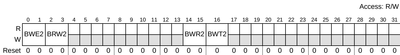
Figure 31-50. Break / Watchpoint Control Register 2 (BWC2)
