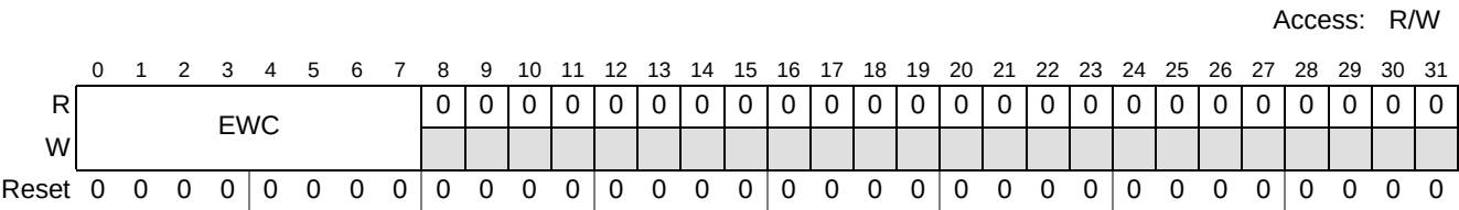
Figure 31-44. Development Control Register 2 (DC2)
