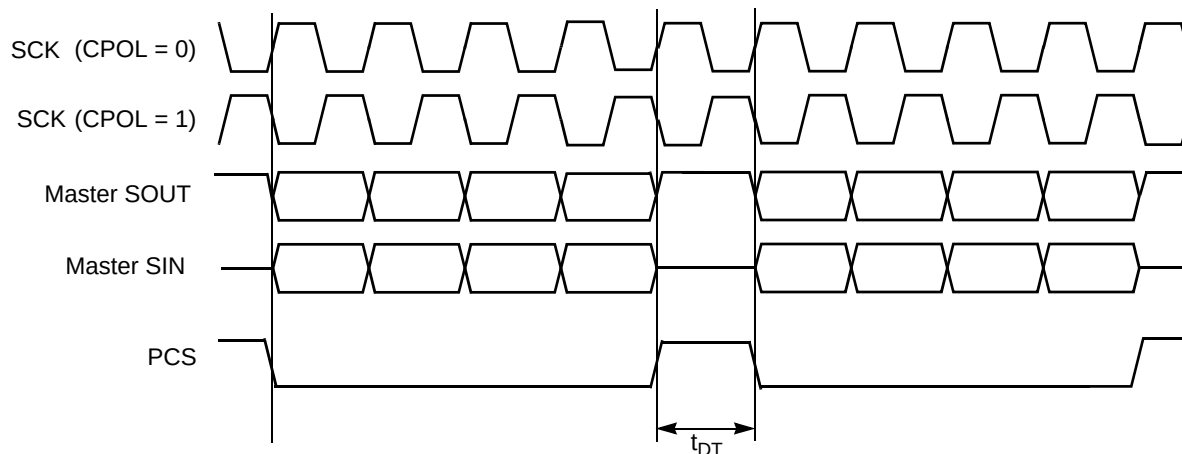
Figure 25-35. Continuous SCK Timing Diagram (CONT=0)
