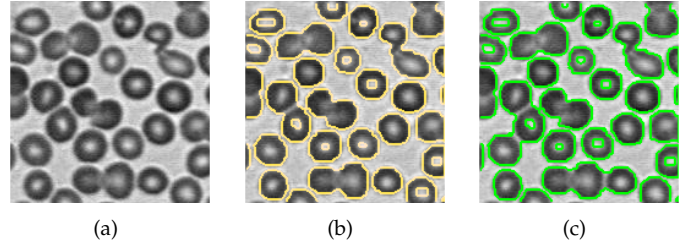
Fig. 6. Unseeded segmentation using unary terms. (a) Original image of blood cells, (b) graph cuts (c) Maximum Spanning Forest (watershed).
