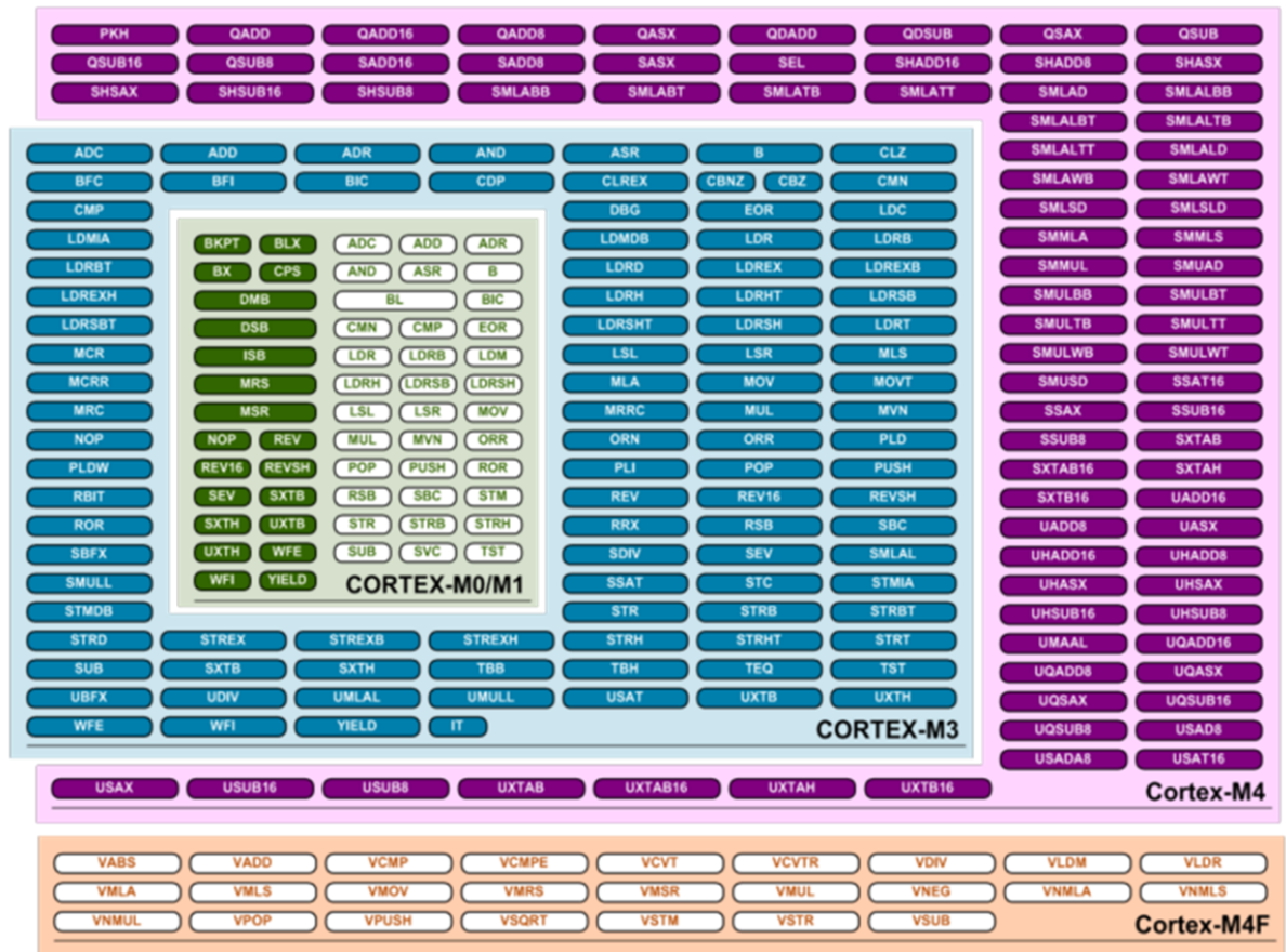
Figure 1-1. Cortex-M Extensions
